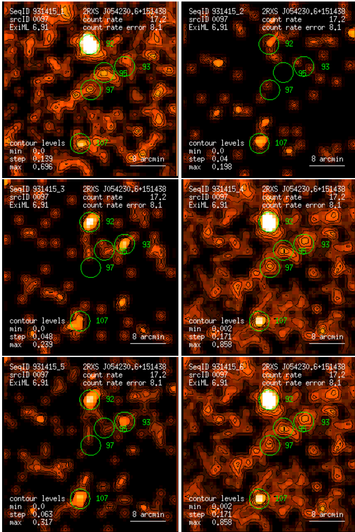
Figure 97: RASS 931415: detection 0097: band rate images, Gaussian filter: (1) PSPC channels 11 – 41, (2) 52 – 90, (3) 91 – 201, (4) 11 – 235, (5) 52 – 201, (6) 11 – 201. Broad band rates in counts/ks. Band rate contour levels in counts/ks/arcmin 2 .
