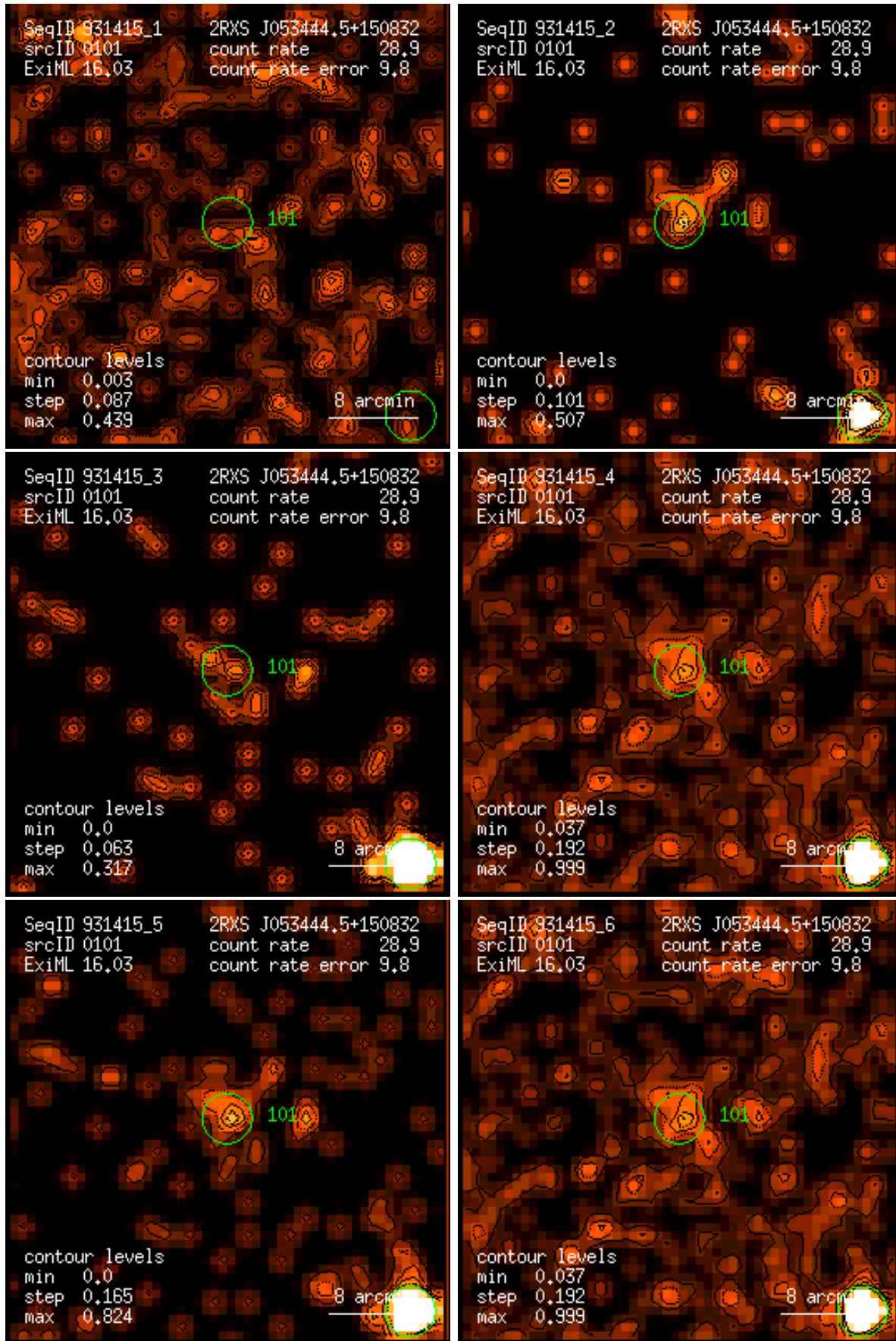
Figure 101: RASS 931415: detection 0101: band rate images, Gaussian filter: (1) PSPC channels 11 – 41, (2) 52 – 90, (3) 91 – 201, (4) 11 – 235, (5) 52 – 201, (6) 11 – 201. Broad band rates in counts/ks. Band rate contour levels in counts/ks/arcmin 2 .
