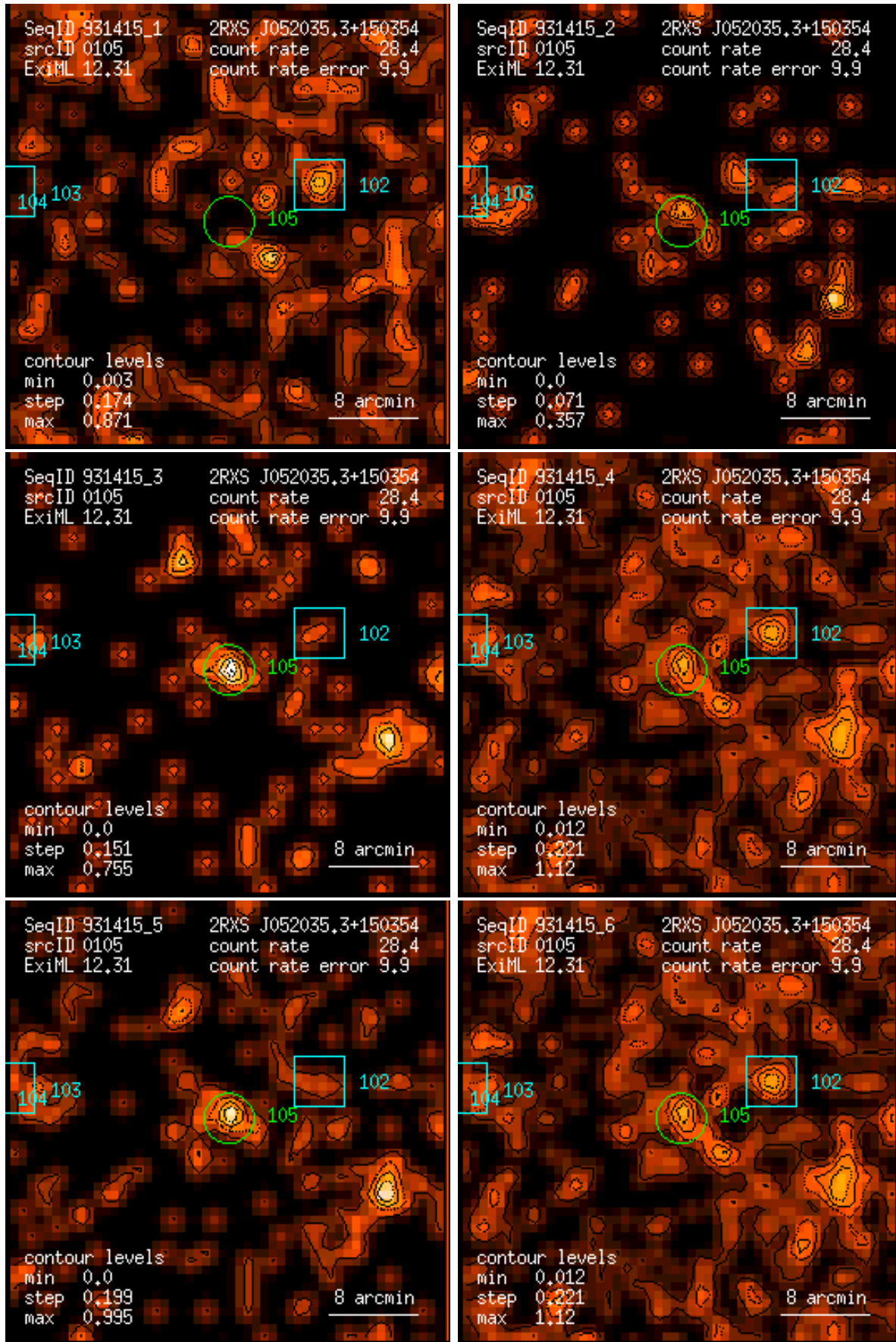
Figure 105: RASS 931415: detection 0105: band rate images, Gaussian filter: (1) PSPC channels 11 – 41, (2) 52 – 90, (3) 91 – 201, (4) 11 – 235, (5) 52 – 201, (6) 11 – 201. Broad band rates in counts/ks. Band rate contour levels in counts/ks/arcmin 2 .
