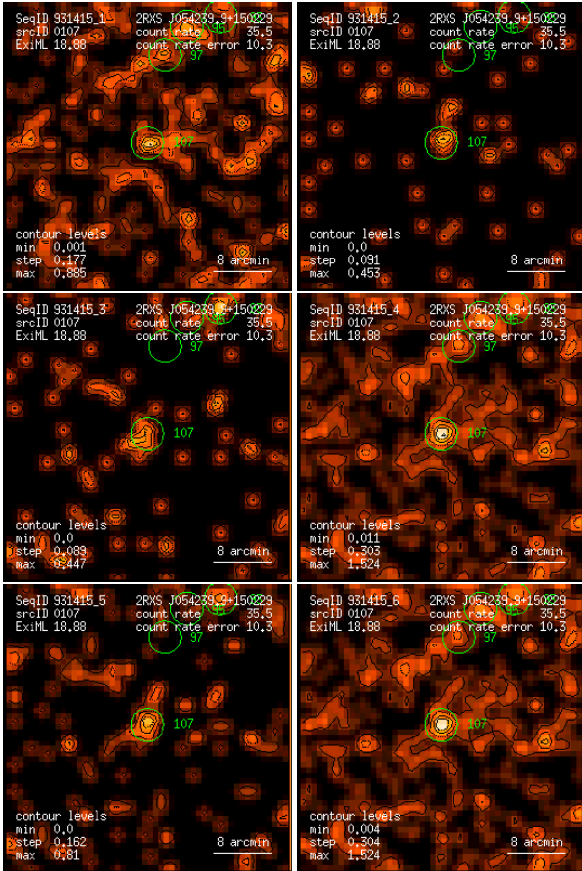
Figure 107: RASS 931415: detection 0107: band rate images, Gaussian filter: (1) PSPC channels 11 – 41, (2) 52 – 90, (3) 91 – 201, (4) 11 – 235, (5) 52 – 201, (6) 11 – 201. Broad band rates in counts/ks. Band rate contour levels in counts/ks/arcmin 2 .
