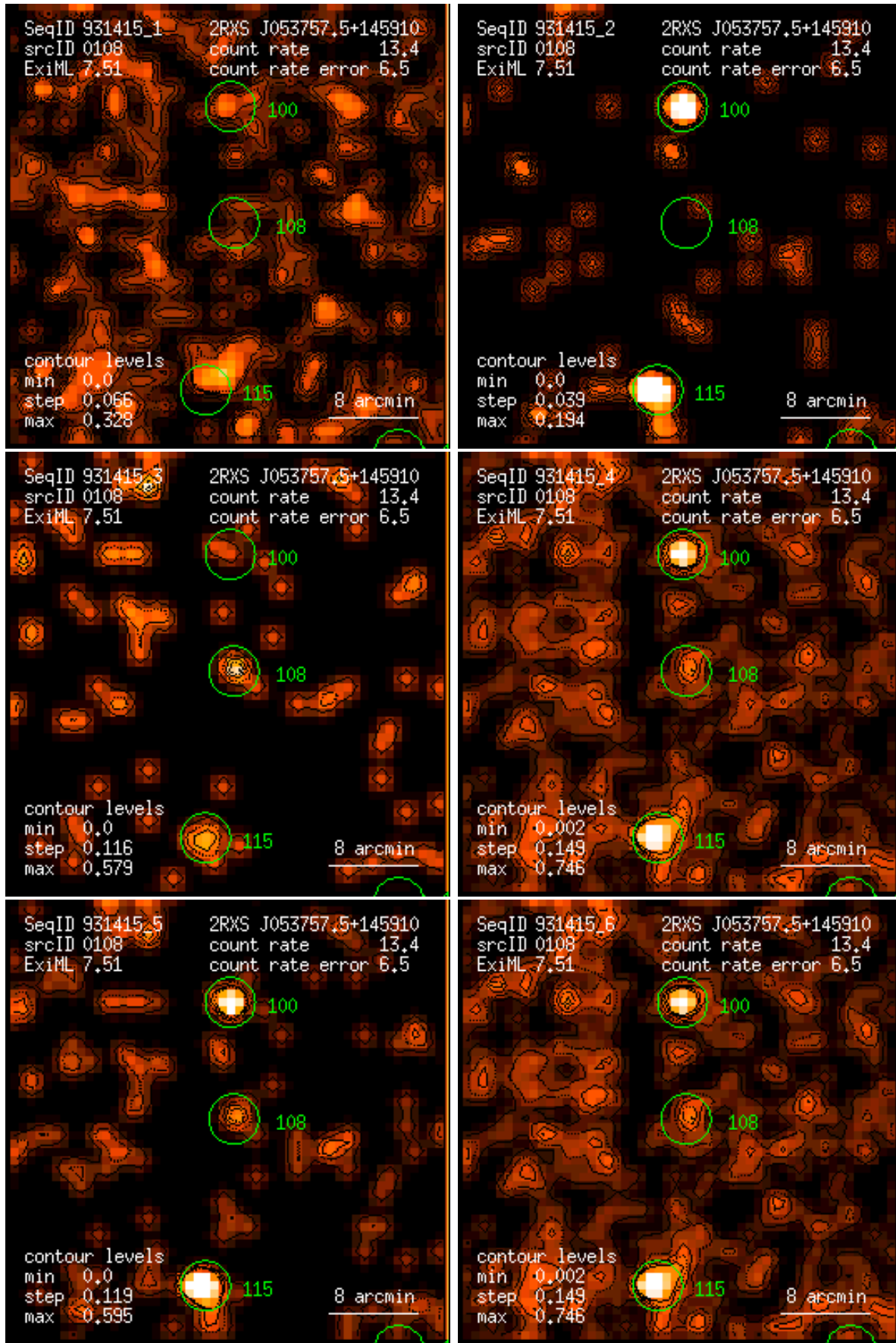
Figure 108: RASS 931415: detection 0108: band rate images, Gaussian filter: (1) PSPC channels 11 – 41, (2) 52 – 90, (3) 91 – 201, (4) 11 – 235, (5) 52 – 201, (6) 11 – 201. Broad band rates in counts/ks. Band rate contour levels in counts/ks/arcmin 2 .
