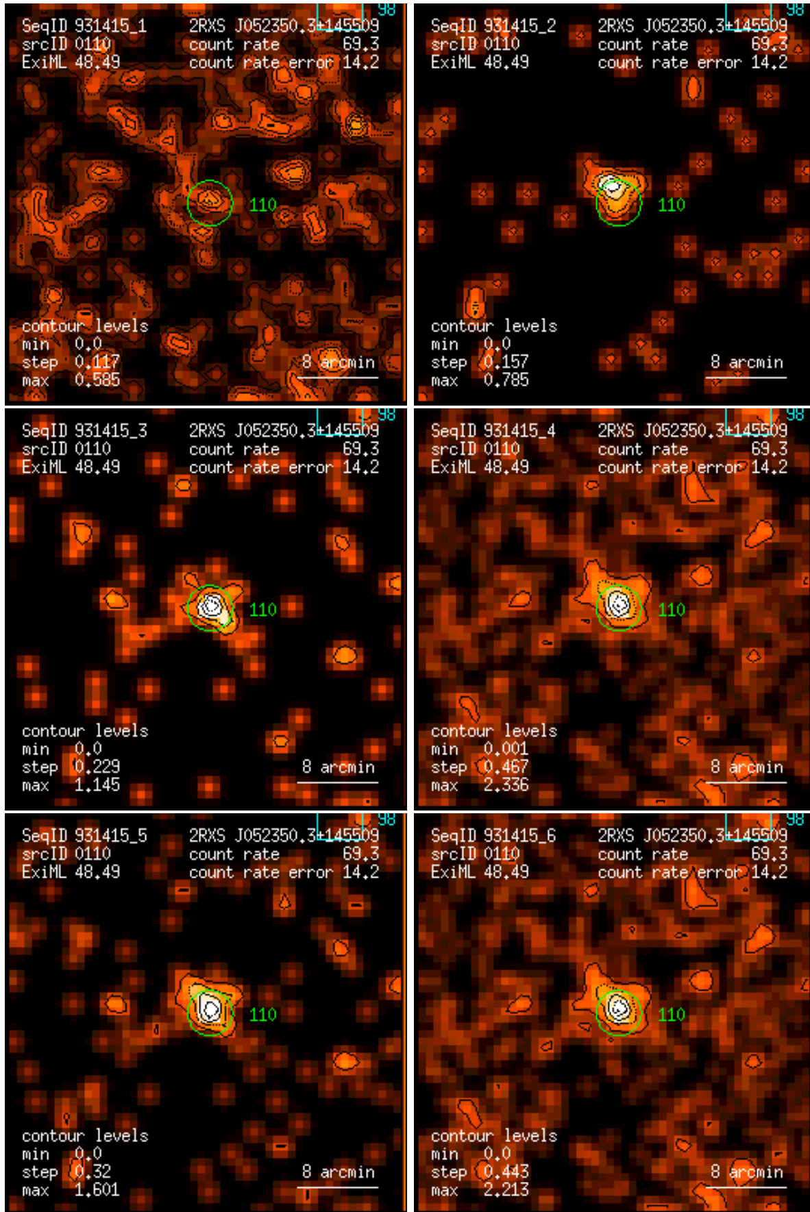
Figure 110: RASS 931415: detection 0110: band rate images, Gaussian filter: (1) PSPC channels 11 – 41, (2) 52 – 90, (3) 91 – 201, (4) 11 – 235, (5) 52 – 201, (6) 11 – 201. Broad band rates in counts/ks. Band rate contour levels in counts/ks/arcmin 2 .
