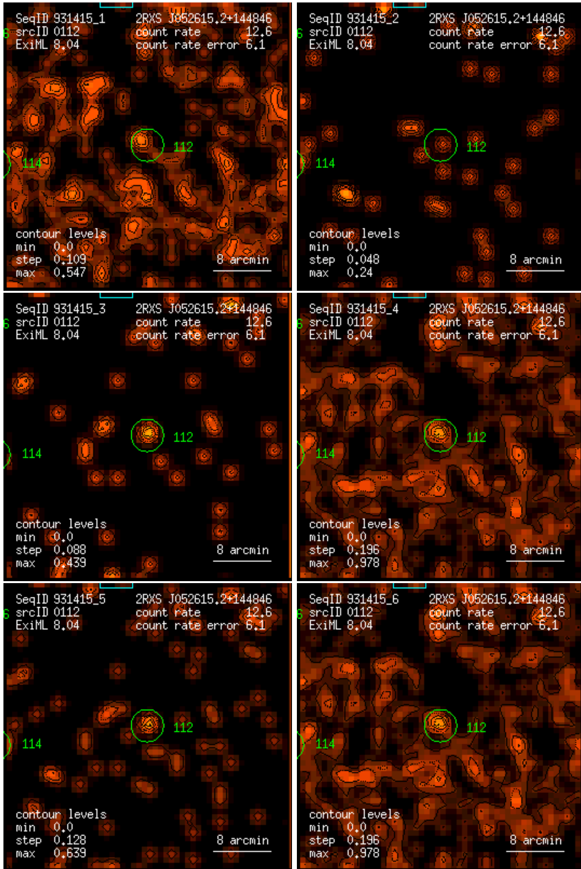
Figure 112: RASS 931415: detection 0112: band rate images, Gaussian filter: (1) PSPC channels 11 – 41, (2) 52 – 90, (3) 91 – 201, (4) 11 – 235, (5) 52 – 201, (6) 11 – 201. Broad band rates in counts/ks. Band rate contour levels in counts/ks/arcmin 2 .
