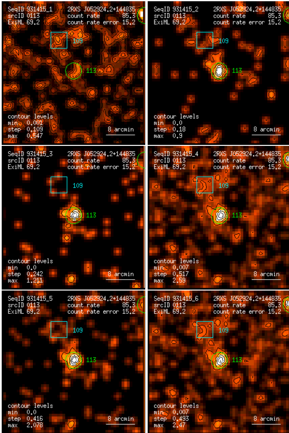
Figure 113: RASS 931415: detection 0113: band rate images, Gaussian filter: (1) PSPC channels 11 – 41, (2) 52 – 90, (3) 91 – 201, (4) 11 – 235, (5) 52 – 201, (6) 11 – 201. Broad band rates in counts/ks. Band rate contour levels in counts/ks/arcmin 2 .
