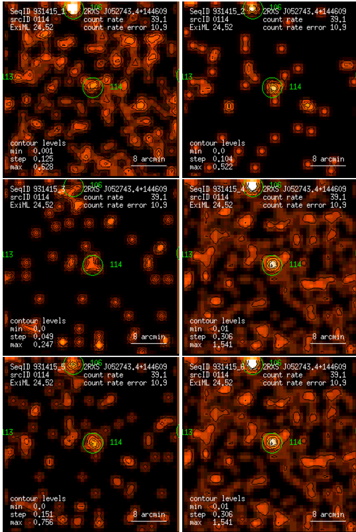
Figure 114: RASS 931415: detection 0114: band rate images, Gaussian filter: (1) PSPC channels 11 – 41, (2) 52 – 90, (3) 91 – 201, (4) 11 – 235, (5) 52 – 201, (6) 11 – 201. Broad band rates in counts/ks. Band rate contour levels in counts/ks/arcmin 2 .
