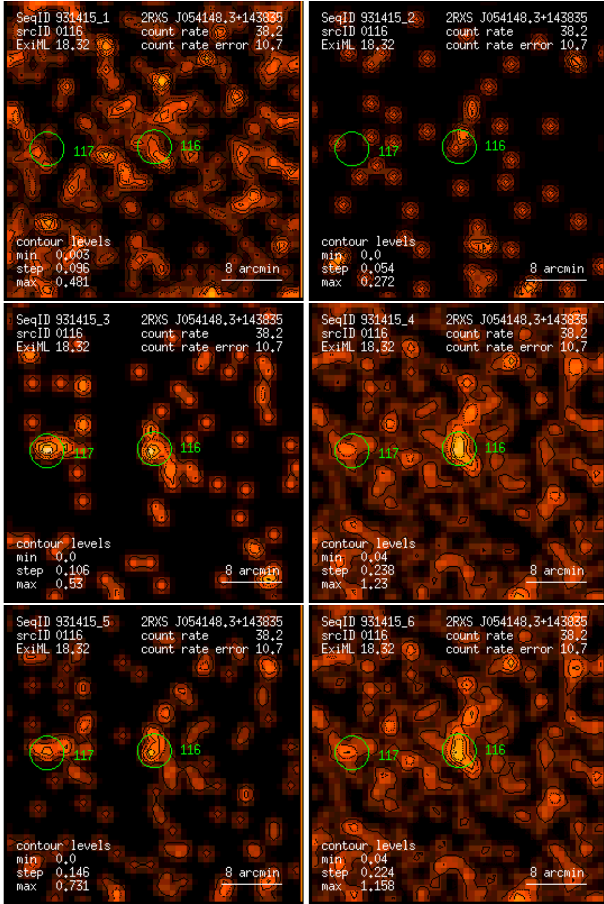
Figure 116: RASS 931415: detection 0116: band rate images, Gaussian filter: (1) PSPC channels 11 – 41, (2) 52 – 90, (3) 91 – 201, (4) 11 – 235, (5) 52 – 201, (6) 11 – 201. Broad band rates in counts/ks. Band rate contour levels in counts/ks/arcmin 2 .
