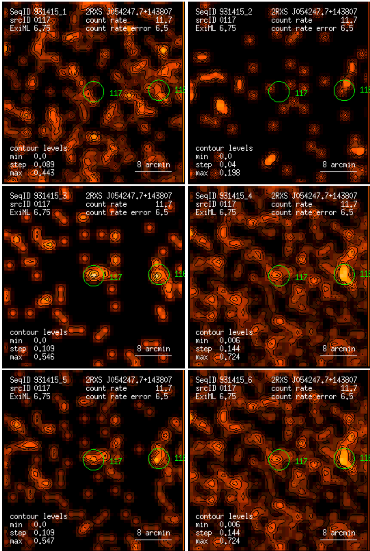
Figure 117: RASS 931415: detection 0117: band rate images, Gaussian filter: (1) PSPC channels 11 – 41, (2) 52 – 90, (3) 91 – 201, (4) 11 – 235, (5) 52 – 201, (6) 11 – 201. Broad band rates in counts/ks. Band rate contour levels in counts/ks/arcmin 2 .
