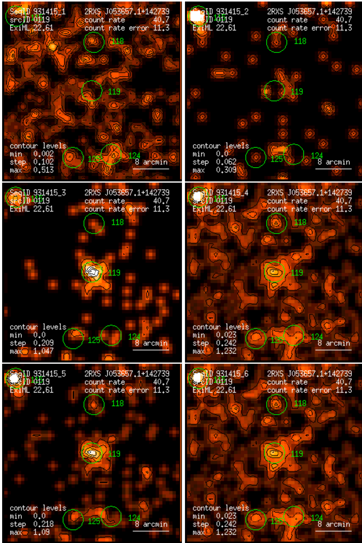
Figure 119: RASS 931415: detection 0119: band rate images, Gaussian filter: (1) PSPC channels 11 – 41, (2) 52 – 90, (3) 91 – 201, (4) 11 – 235, (5) 52 – 201, (6) 11 – 201. Broad band rates in counts/ks. Band rate contour levels in counts/ks/arcmin 2 .
