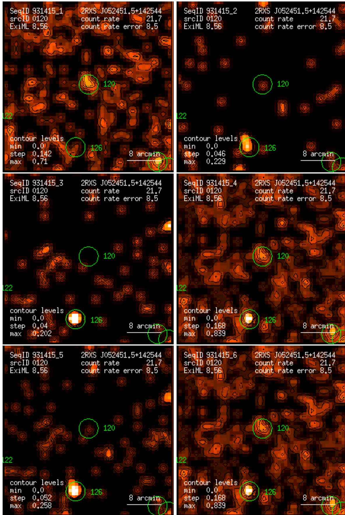
Figure 120: RASS 931415: detection 0120: band rate images, Gaussian filter: (1) PSPC channels 11 – 41, (2) 52 – 90, (3) 91 – 201, (4) 11 – 235, (5) 52 – 201, (6) 11 – 201. Broad band rates in counts/ks. Band rate contour levels in counts/ks/arcmin 2 .
