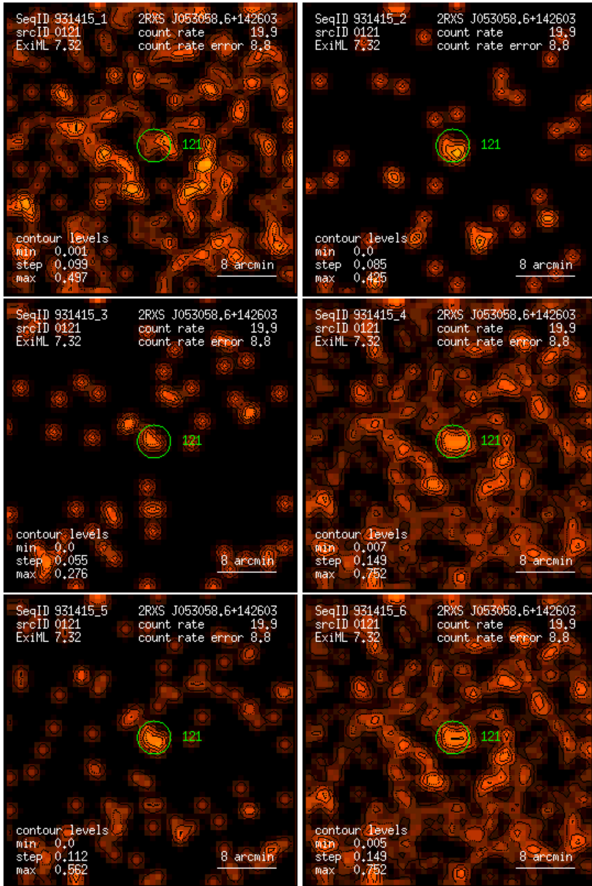
Figure 121: RASS 931415: detection 0121: band rate images, Gaussian filter: (1) PSPC channels 11 – 41, (2) 52 – 90, (3) 91 – 201, (4) 11 – 235, (5) 52 – 201, (6) 11 – 201. Broad band rates in counts/ks. Band rate contour levels in counts/ks/arcmin 2 .
