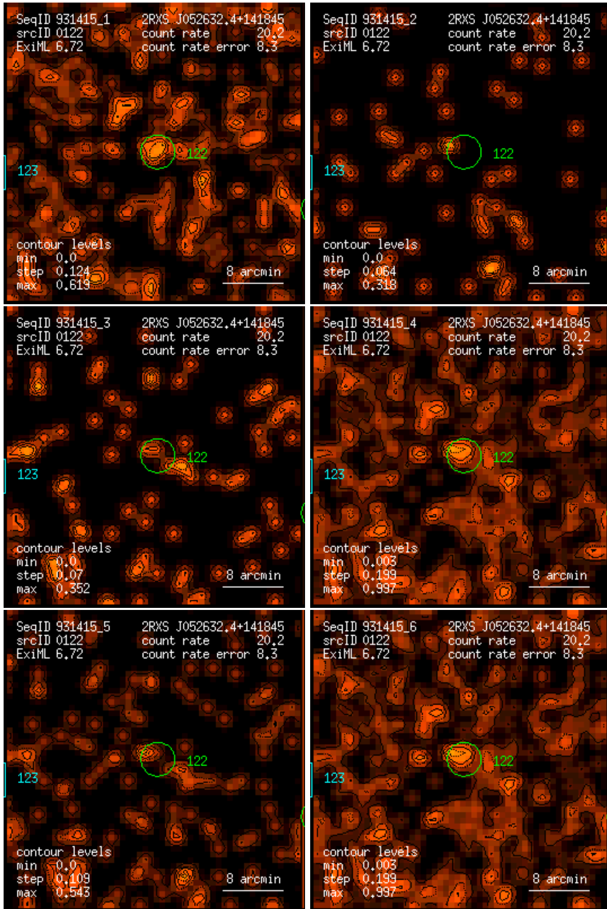
Figure 122: RASS 931415: detection 0122: band rate images, Gaussian filter: (1) PSPC channels 11 – 41, (2) 52 – 90, (3) 91 – 201, (4) 11 – 235, (5) 52 – 201, (6) 11 – 201. Broad band rates in counts/ks. Band rate contour levels in counts/ks/arcmin 2 .
