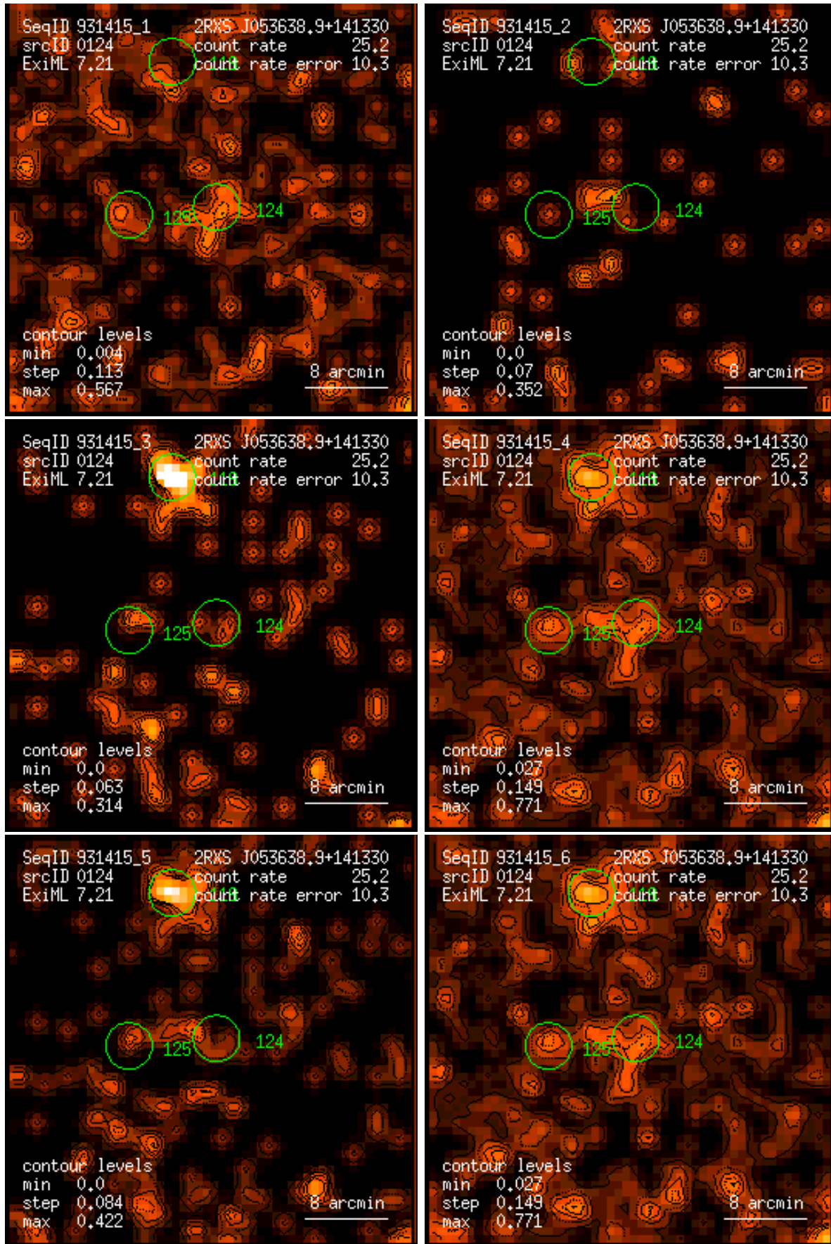
Figure 124: RASS 931415: detection 0124: band rate images, Gaussian filter: (1) PSPC channels 11 – 41, (2) 52 – 90, (3) 91 – 201, (4) 11 – 235, (5) 52 – 201, (6) 11 – 201. Broad band rates in counts/ks. Band rate contour levels in counts/ks/arcmin 2 .
