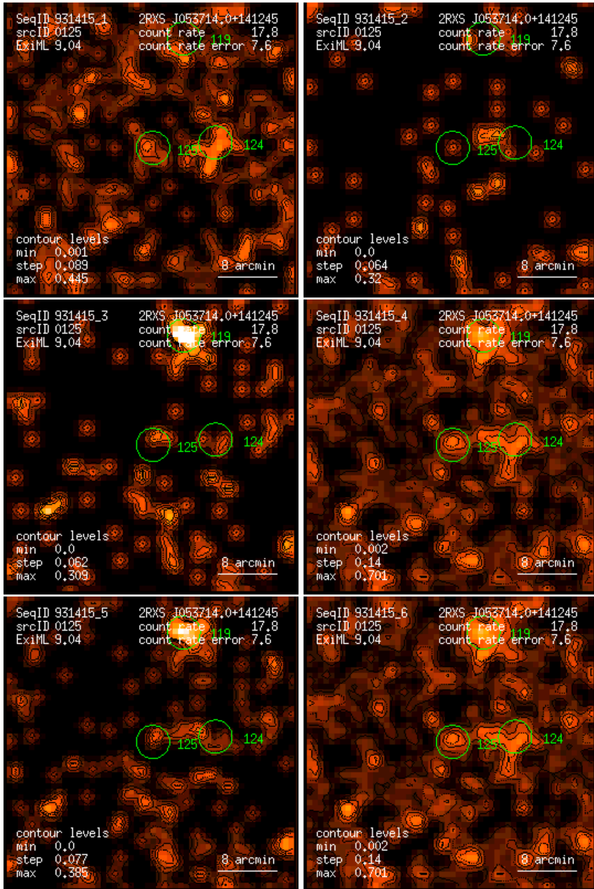
Figure 125: RASS 931415: detection 0125: band rate images, Gaussian filter: (1) PSPC channels 11 – 41, (2) 52 – 90, (3) 91 – 201, (4) 11 – 235, (5) 52 – 201, (6) 11 – 201. Broad band rates in counts/ks. Band rate contour levels in counts/ks/arcmin 2 .
