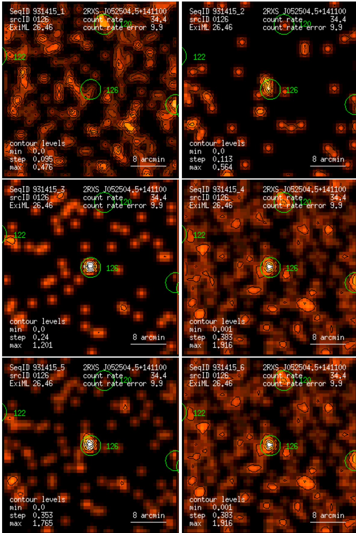
Figure 126: RASS 931415: detection 0126: band rate images, Gaussian filter: (1) PSPC channels 11 – 41, (2) 52 – 90, (3) 91 – 201, (4) 11 – 235, (5) 52 – 201, (6) 11 – 201. Broad band rates in counts/ks. Band rate contour levels in counts/ks/arcmin 2 .
