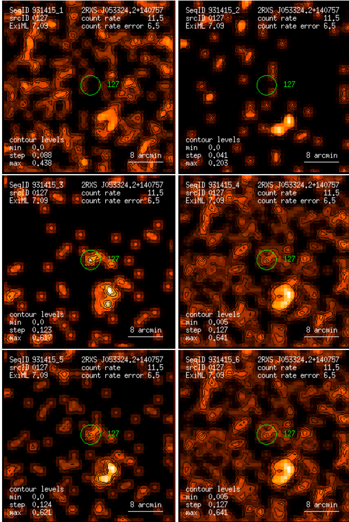
Figure 127: RASS 931415: detection 0127: band rate images, Gaussian filter: (1) PSPC channels 11 – 41, (2) 52 – 90, (3) 91 – 201, (4) 11 – 235, (5) 52 – 201, (6) 11 – 201. Broad band rates in counts/ks. Band rate contour levels in counts/ks/arcmin 2 .
