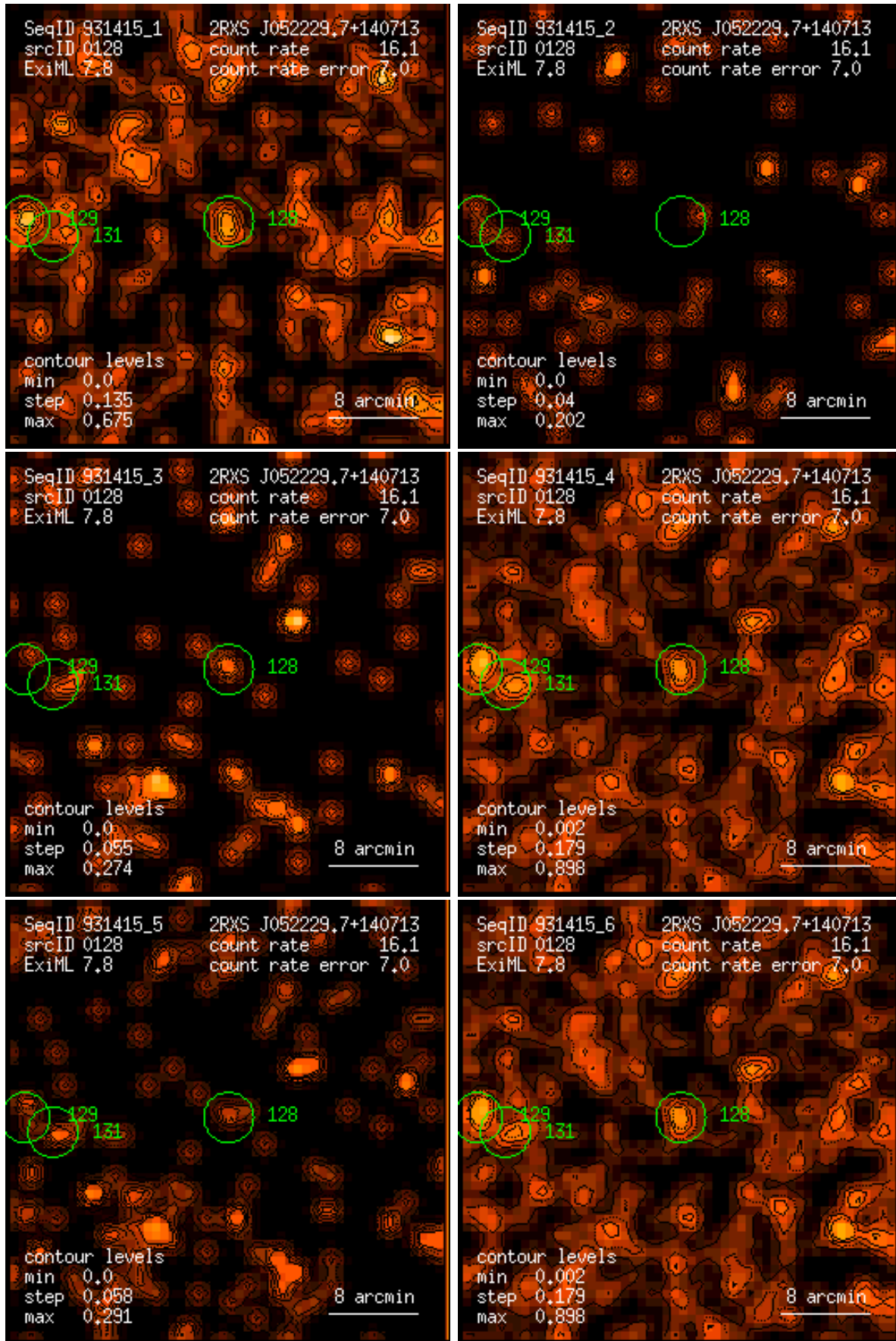
Figure 128: RASS 931415: detection 0128: band rate images, Gaussian filter: (1) PSPC channels 11 – 41, (2) 52 – 90, (3) 91 – 201, (4) 11 – 235, (5) 52 – 201, (6) 11 – 201. Broad band rates in counts/ks. Band rate contour levels in counts/ks/arcmin 2 .
