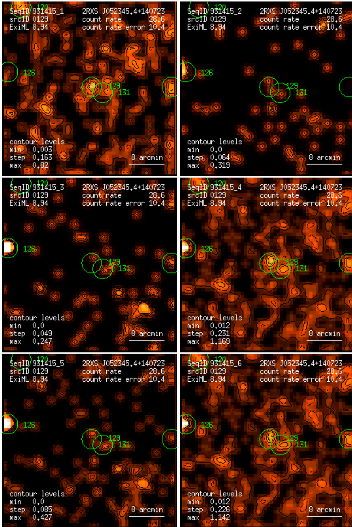
Figure 129: RASS 931415: detection 0129: band rate images, Gaussian filter: (1) PSPC channels 11 – 41, (2) 52 – 90, (3) 91 – 201, (4) 11 – 235, (5) 52 – 201, (6) 11 – 201. Broad band rates in counts/ks. Band rate contour levels in counts/ks/arcmin 2 .
