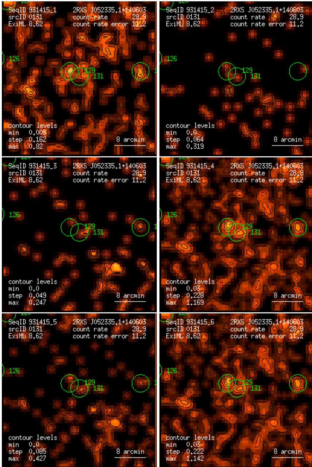
Figure 131: RASS 931415: detection 0131: band rate images, Gaussian filter: (1) PSPC channels 11 – 41, (2) 52 – 90, (3) 91 – 201, (4) 11 – 235, (5) 52 – 201, (6) 11 – 201. Broad band rates in counts/ks. Band rate contour levels in counts/ks/arcmin 2 .
