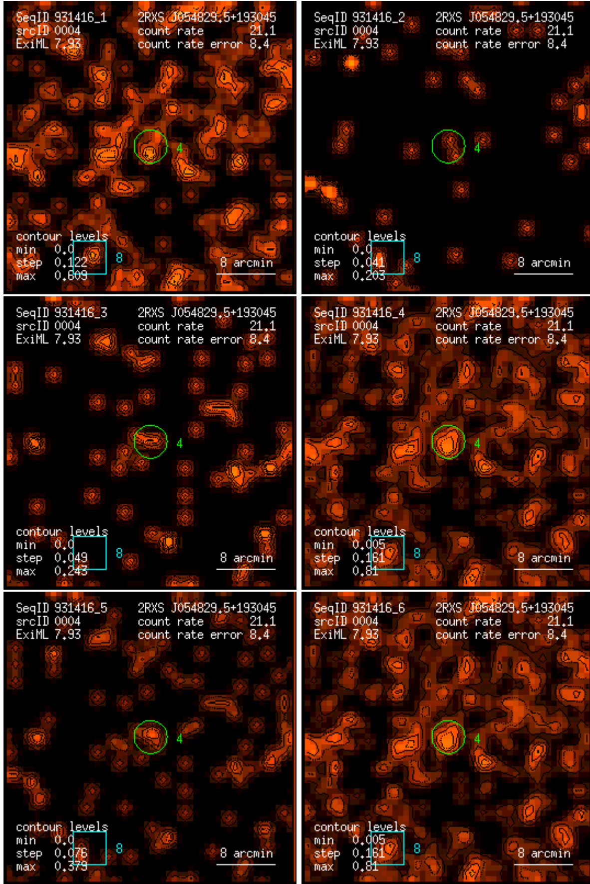
Figure 4: RASS 931416: detection 0004: band rate images, Gaussian filter: (1) PSPC channels 11 – 41, (2) 52 – 90, (3) 91 – 201, (4) 11 – 235, (5) 52 – 201, (6) 11 – 201. Broad band rates in counts/ks. Band rate contour levels in counts/ks/arcmin 2 .
