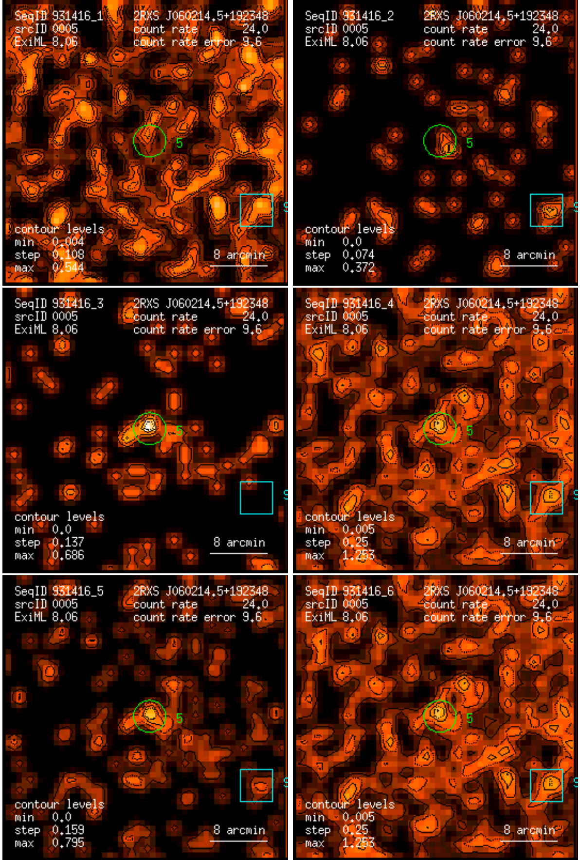
Figure 5: RASS 931416: detection 0005: band rate images, Gaussian filter: (1) PSPC channels 11 – 41, (2) 52 – 90, (3) 91 – 201, (4) 11 – 235, (5) 52 – 201, (6) 11 – 201. Broad band rates in counts/ks. Band rate contour levels in counts/ks/arcmin 2 .
