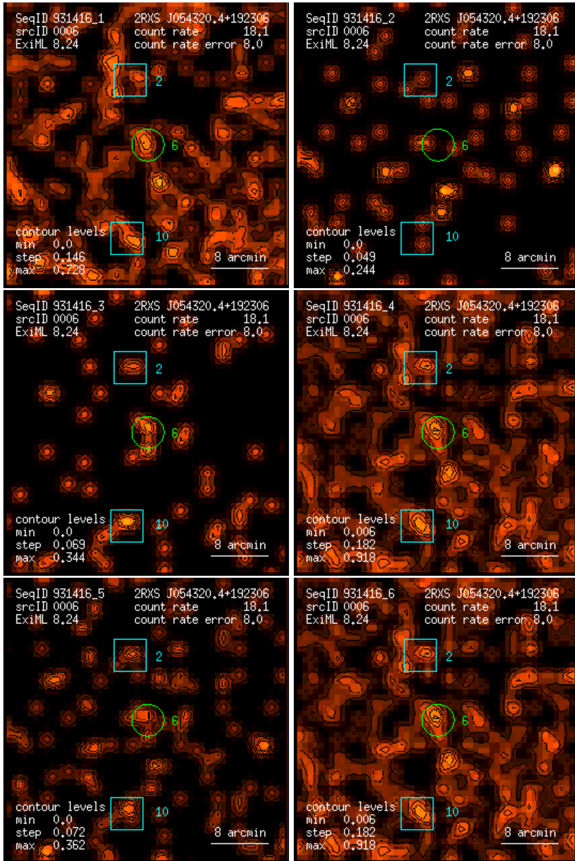
Figure 6: RASS 931416: detection 0006: band rate images, Gaussian filter: (1) PSPC channels 11 – 41, (2) 52 – 90, (3) 91 – 201, (4) 11 – 235, (5) 52 – 201, (6) 11 – 201. Broad band rates in counts/ks. Band rate contour levels in counts/ks/arcmin 2 .
