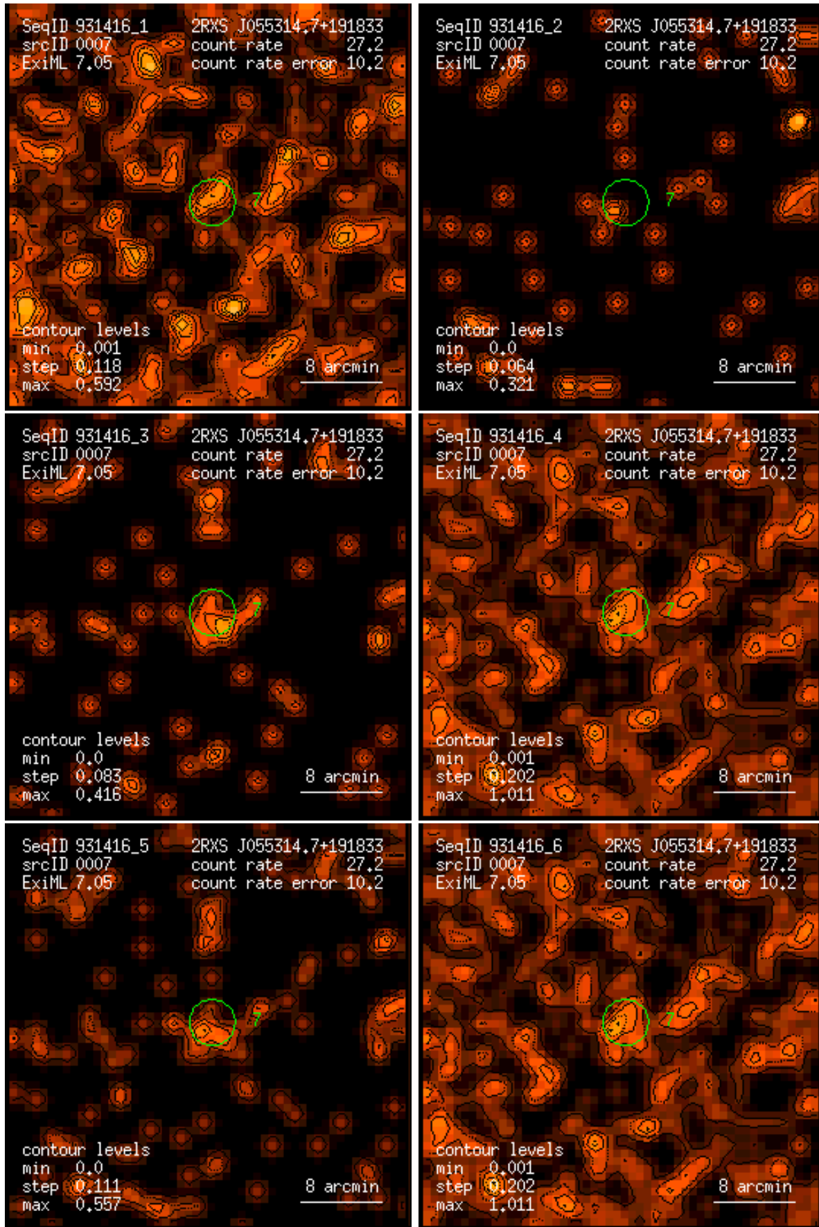
Figure 7: RASS 931416: detection 0007: band rate images, Gaussian filter: (1) PSPC channels 11 – 41, (2) 52 – 90, (3) 91 – 201, (4) 11 – 235, (5) 52 – 201, (6) 11 – 201. Broad band rates in counts/ks. Band rate contour levels in counts/ks/arcmin 2 .
