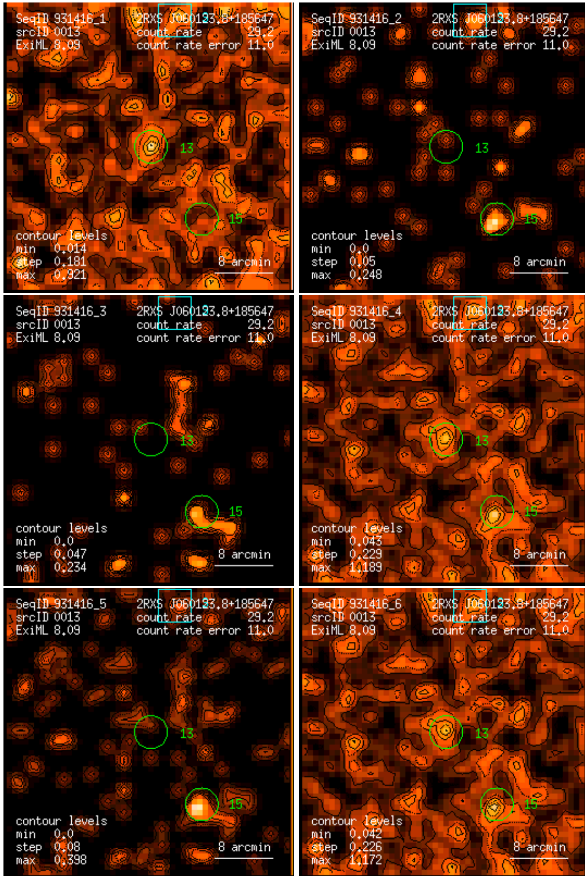
Figure 13: RASS 931416: detection 0013: band rate images, Gaussian filter: (1) PSPC channels 11 – 41, (2) 52 – 90, (3) 91 – 201, (4) 11 – 235, (5) 52 – 201, (6) 11 – 201. Broad band rates in counts/ks. Band rate contour levels in counts/ks/arcmin 2 .
