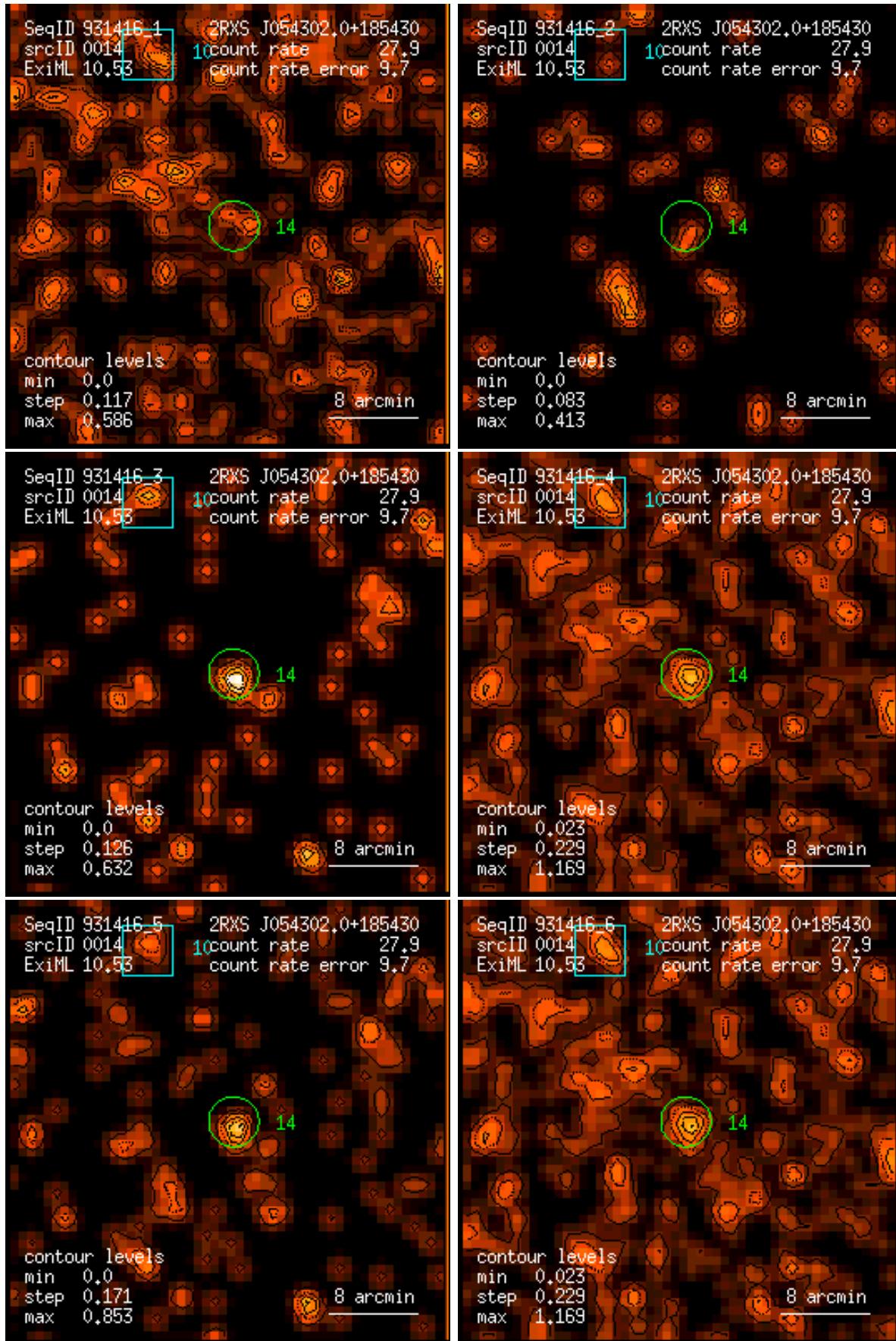
Figure 14: RASS 931416: detection 0014: band rate images, Gaussian filter: (1) PSPC channels 11 – 41, (2) 52 – 90, (3) 91 – 201, (4) 11 – 235, (5) 52 – 201, (6) 11 – 201. Broad band rates in counts/ks. Band rate contour levels in counts/ks/arcmin 2 .
