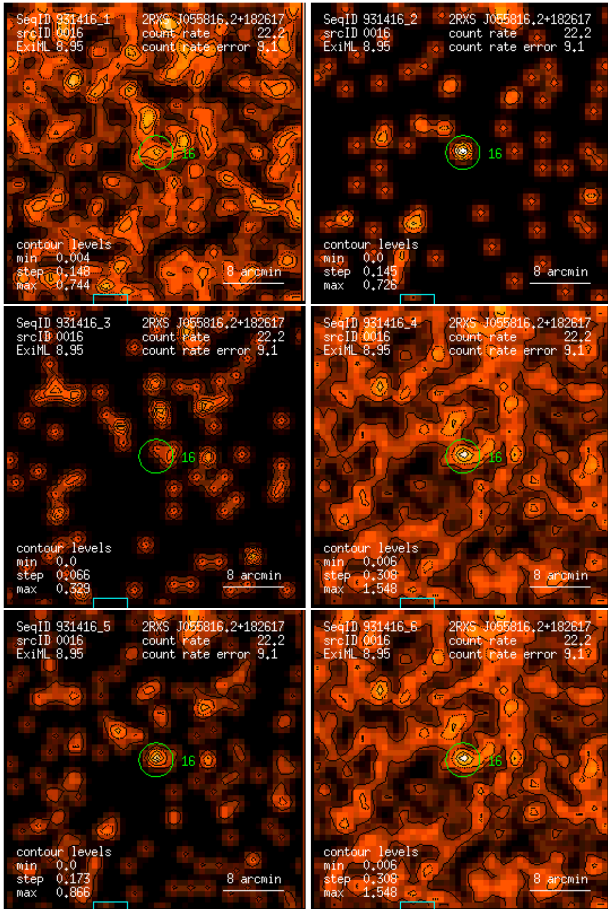
Figure 16: RASS 931416: detection 0016: band rate images, Gaussian filter: (1) PSPC channels 11 – 41, (2) 52 – 90, (3) 91 – 201, (4) 11 – 235, (5) 52 – 201, (6) 11 – 201. Broad band rates in counts/ks. Band rate contour levels in counts/ks/arcmin 2 .
