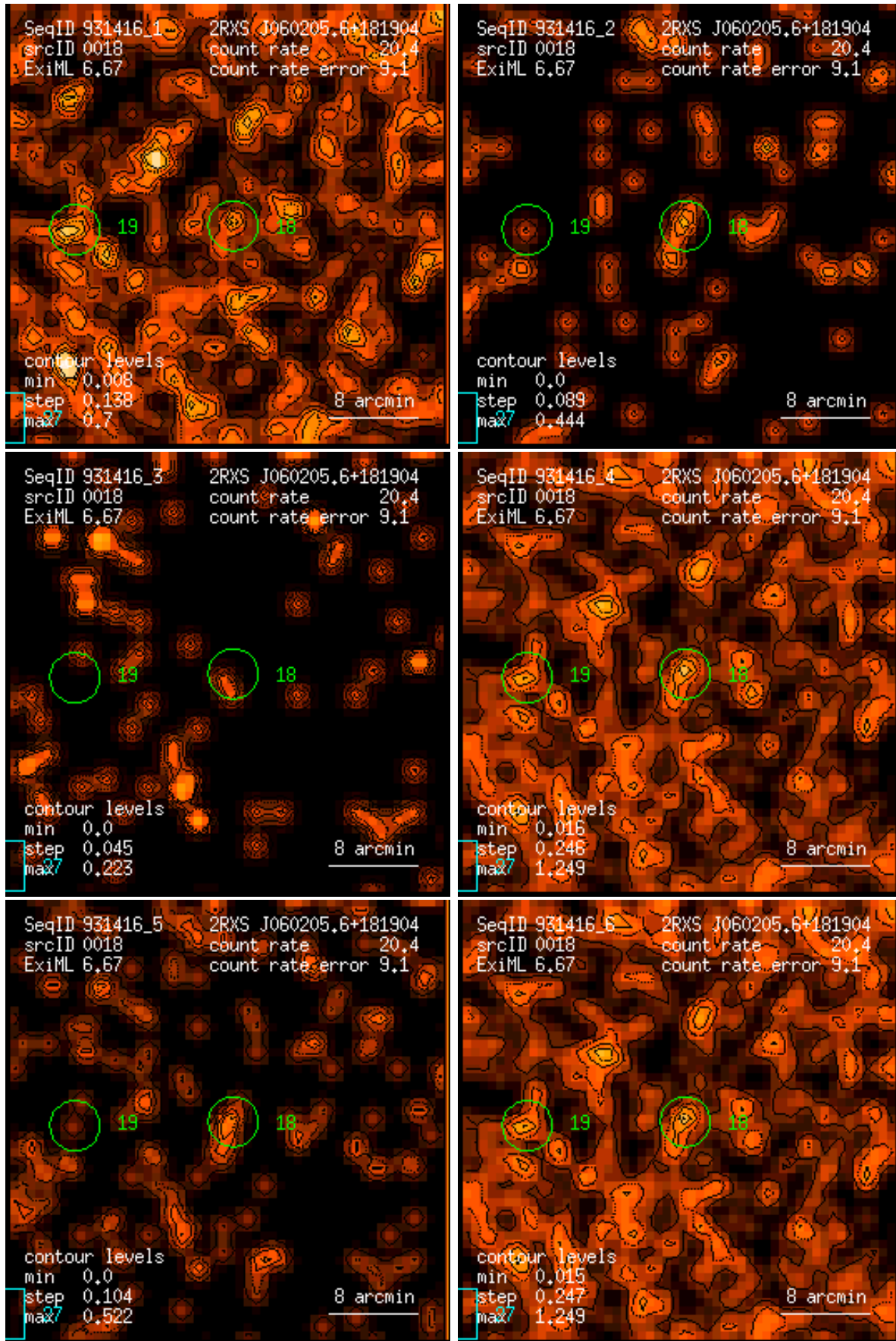
Figure 18: RASS 931416: detection 0018: band rate images, Gaussian filter: (1) PSPC channels 11 – 41, (2) 52 – 90, (3) 91 – 201, (4) 11 – 235, (5) 52 – 201, (6) 11 – 201. Broad band rates in counts/ks. Band rate contour levels in counts/ks/arcmin 2 .
