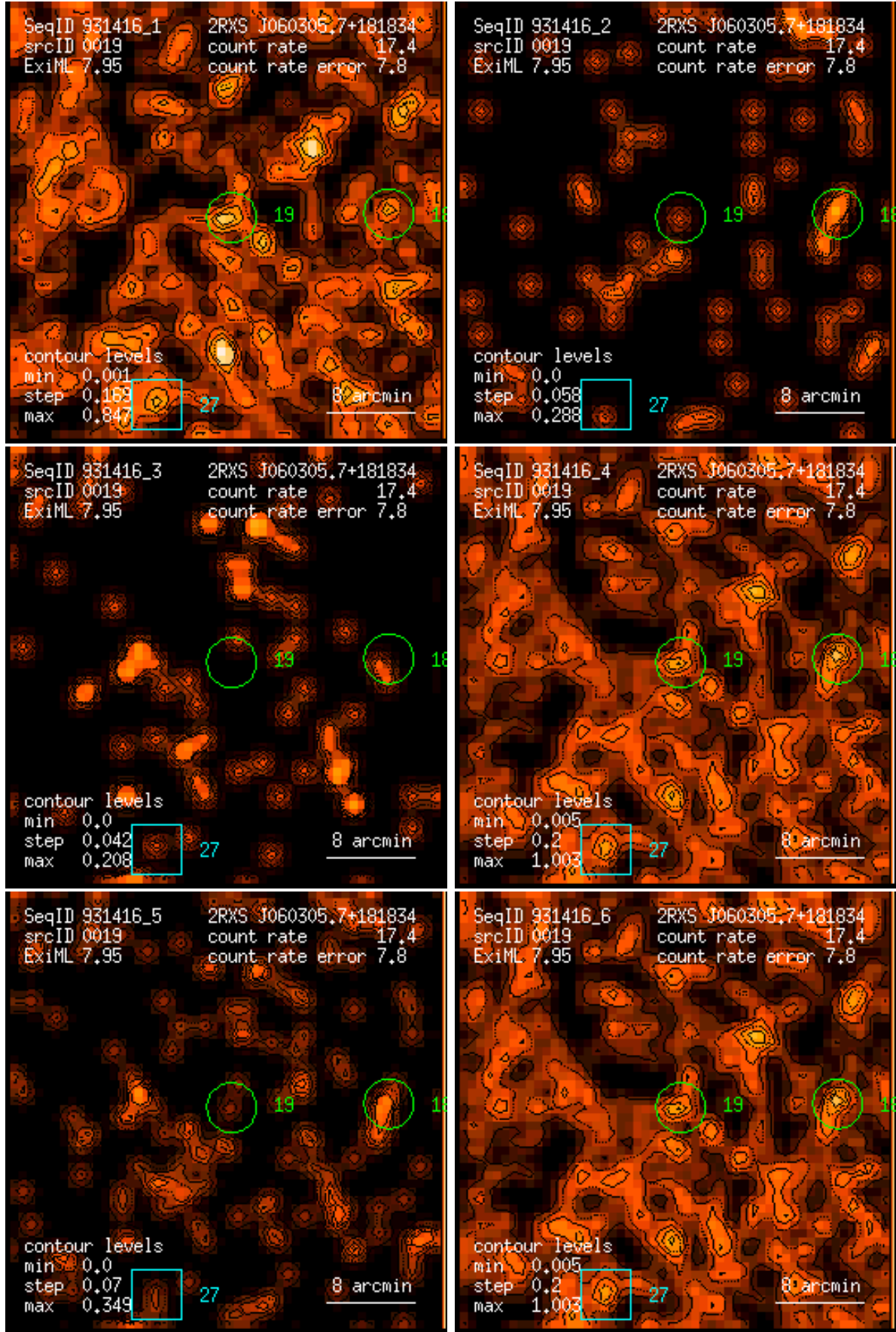
Figure 19: RASS 931416: detection 0019: band rate images, Gaussian filter: (1) PSPC channels 11 – 41, (2) 52 – 90, (3) 91 – 201, (4) 11 – 235, (5) 52 – 201, (6) 11 – 201. Broad band rates in counts/ks. Band rate contour levels in counts/ks/arcmin 2 .
