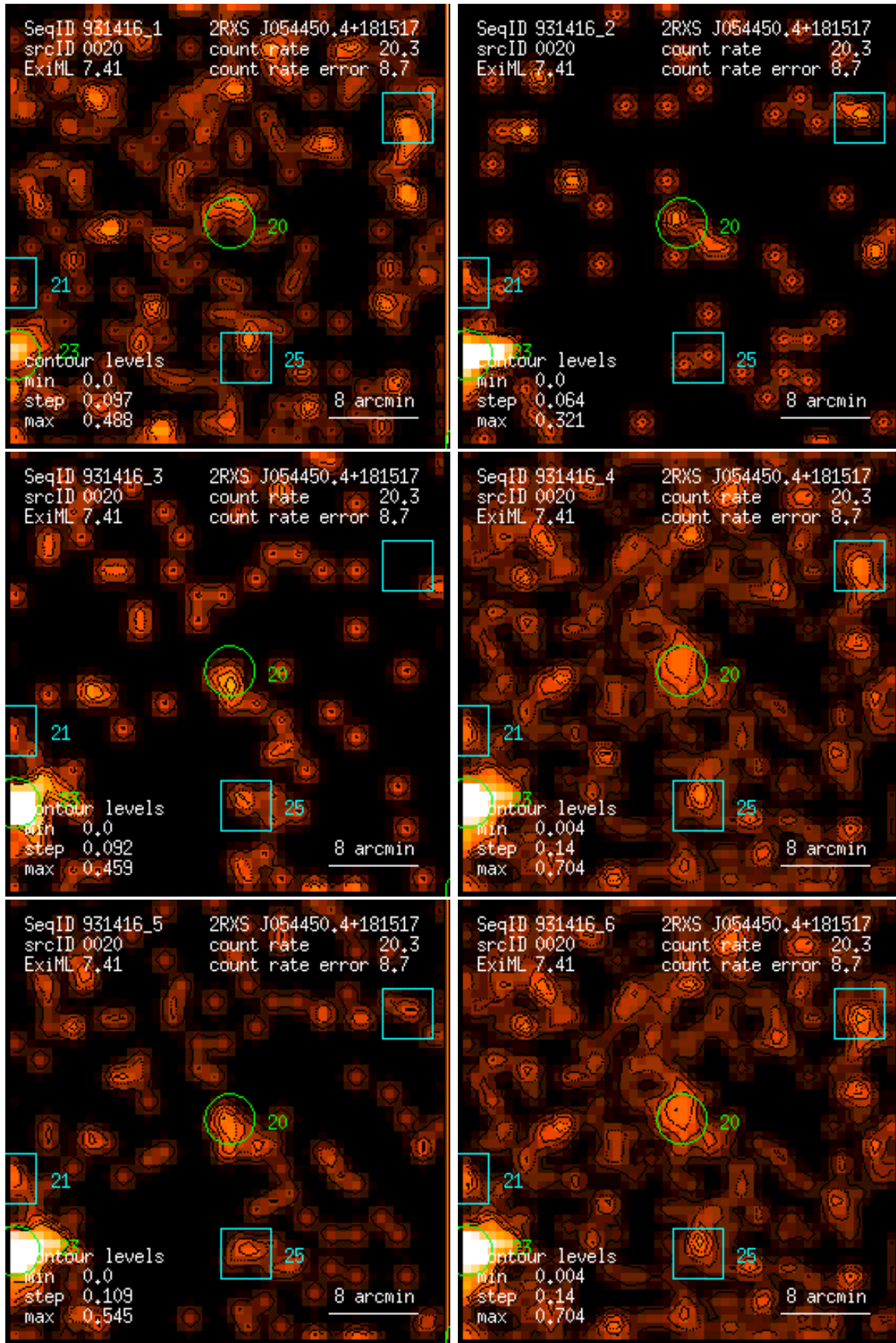
Figure 20: RASS 931416: detection 0020: band rate images, Gaussian filter: (1) PSPC channels 11 – 41, (2) 52 – 90, (3) 91 – 201, (4) 11 – 235, (5) 52 – 201, (6) 11 – 201. Broad band rates in counts/ks. Band rate contour levels in counts/ks/arcmin 2 .
