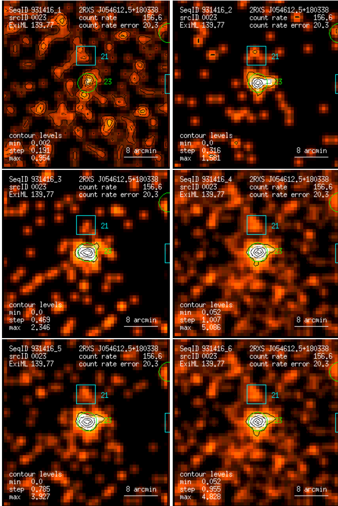
Figure 23: RASS 931416: detection 0023: band rate images, Gaussian filter: (1) PSPC channels 11 – 41, (2) 52 – 90, (3) 91 – 201, (4) 11 – 235, (5) 52 – 201, (6) 11 – 201. Broad band rates in counts/ks. Band rate contour levels in counts/ks/arcmin 2 .
