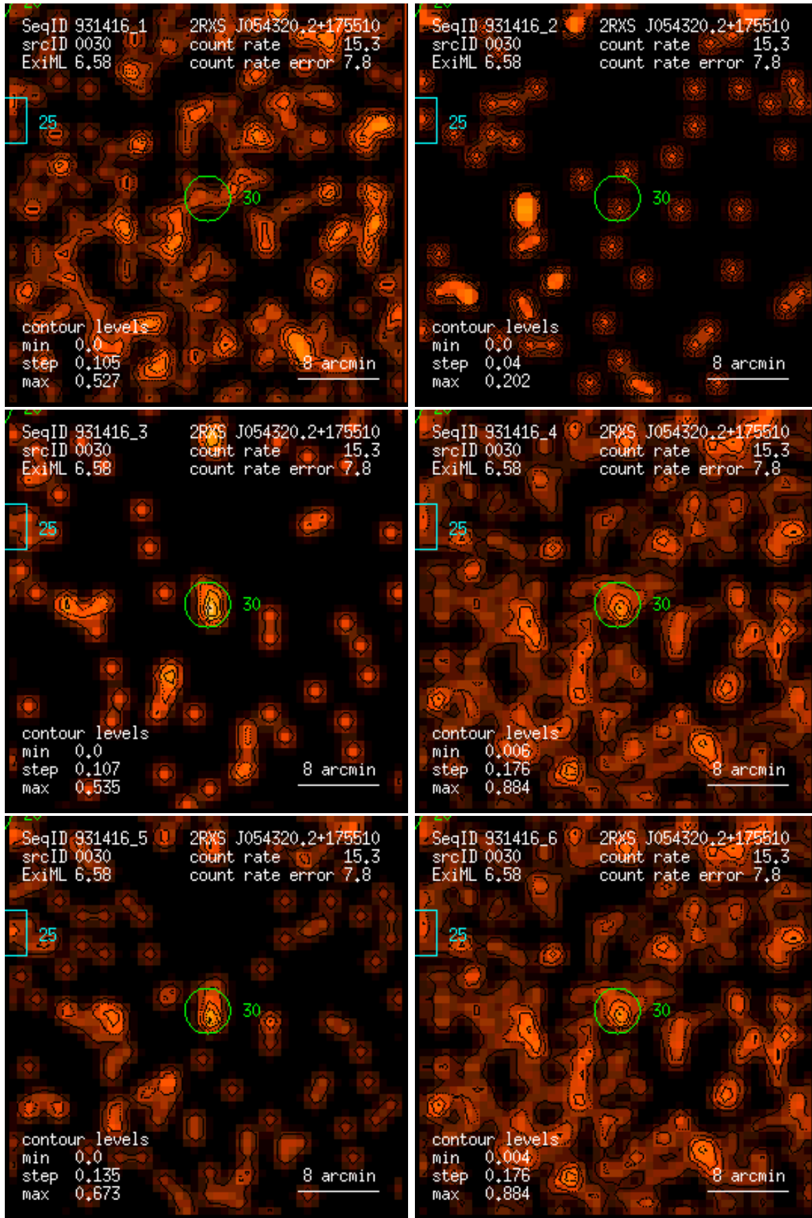
Figure 30: RASS 931416: detection 0030: band rate images, Gaussian filter: (1) PSPC channels 11 – 41, (2) 52 – 90, (3) 91 – 201, (4) 11 – 235, (5) 52 – 201, (6) 11 – 201. Broad band rates in counts/ks. Band rate contour levels in counts/ks/arcmin 2 .
