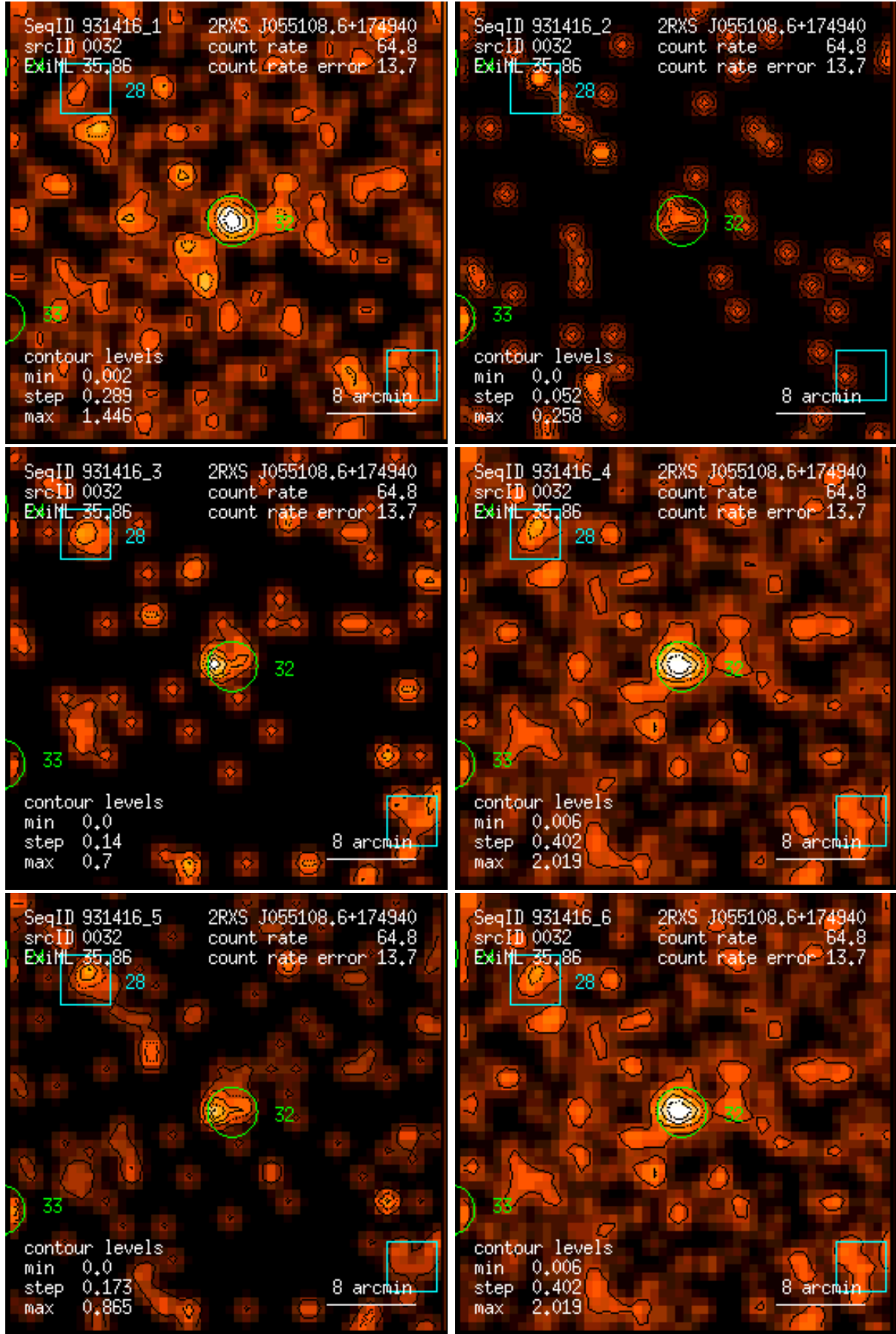
Figure 32: RASS 931416: detection 0032: band rate images, Gaussian filter: (1) PSPC channels 11 – 41, (2) 52 – 90, (3) 91 – 201, (4) 11 – 235, (5) 52 – 201, (6) 11 – 201. Broad band rates in counts/ks. Band rate contour levels in counts/ks/arcmin 2 .
