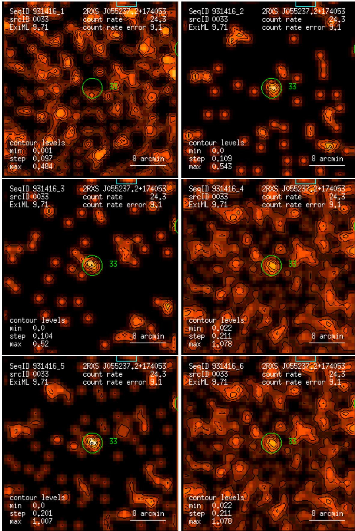
Figure 33: RASS 931416: detection 0033: band rate images, Gaussian filter: (1) PSPC channels 11 – 41, (2) 52 – 90, (3) 91 – 201, (4) 11 – 235, (5) 52 – 201, (6) 11 – 201. Broad band rates in counts/ks. Band rate contour levels in counts/ks/arcmin 2 .
