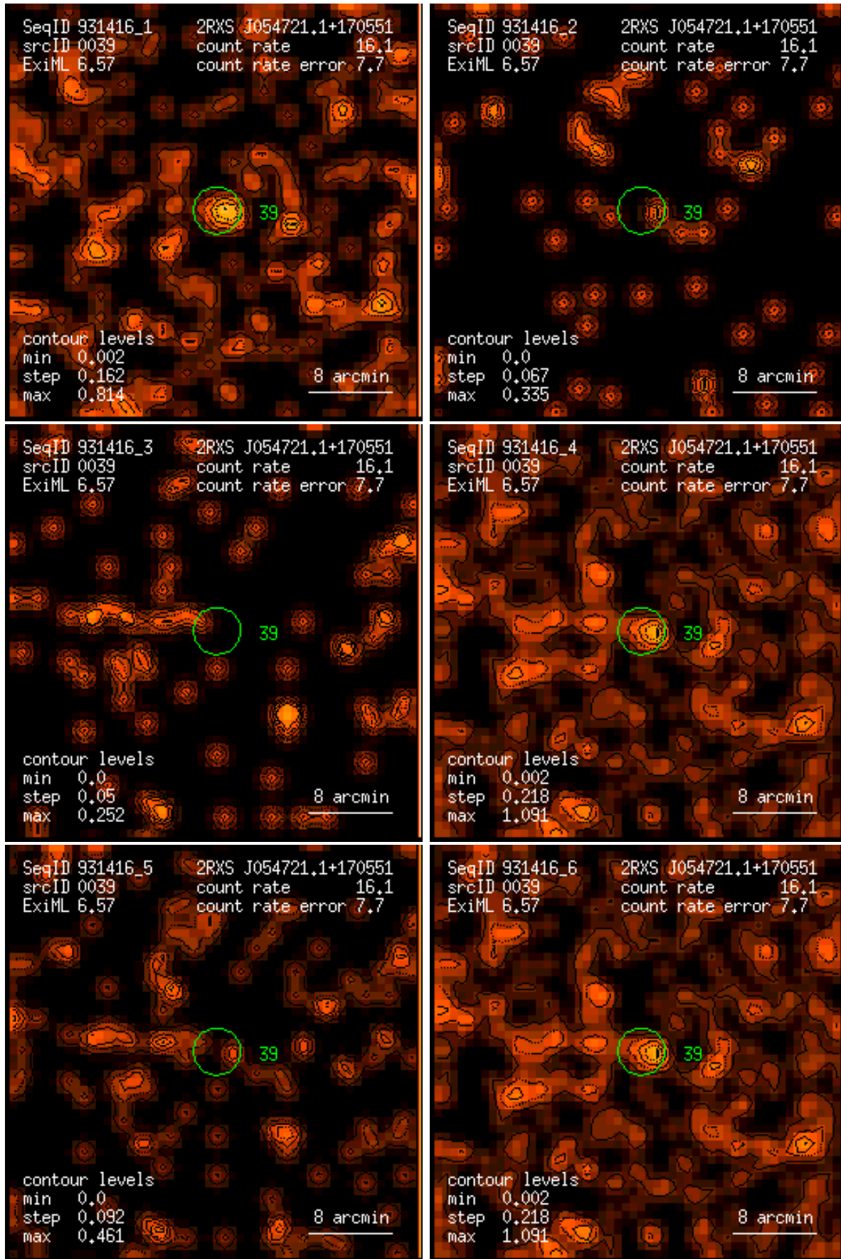
Figure 39: RASS 931416: detection 0039: band rate images, Gaussian filter: (1) PSPC channels 11 – 41, (2) 52 – 90, (3) 91 – 201, (4) 11 – 235, (5) 52 – 201, (6) 11 – 201. Broad band rates in counts/ks. Band rate contour levels in counts/ks/arcmin 2 .
