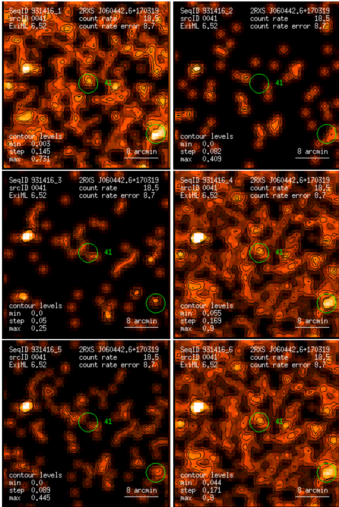
Figure 41: RASS 931416: detection 0041: band rate images, Gaussian filter: (1) PSPC channels 11 – 41, (2) 52 – 90, (3) 91 – 201, (4) 11 – 235, (5) 52 – 201, (6) 11 – 201. Broad band rates in counts/ks. Band rate contour levels in counts/ks/arcmin 2 .
