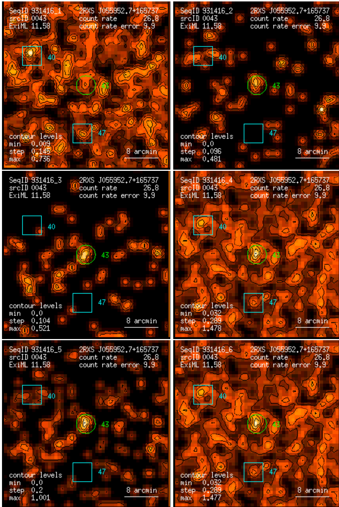
Figure 43: RASS 931416: detection 0043: band rate images, Gaussian filter: (1) PSPC channels 11 – 41, (2) 52 – 90, (3) 91 – 201, (4) 11 – 235, (5) 52 – 201, (6) 11 – 201. Broad band rates in counts/ks. Band rate contour levels in counts/ks/arcmin 2 .
