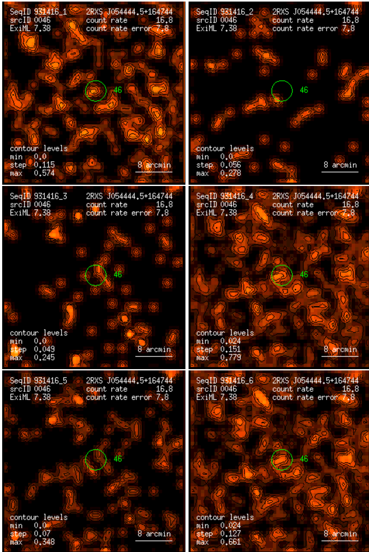
Figure 46: RASS 931416: detection 0046: band rate images, Gaussian filter: (1) PSPC channels 11 – 41, (2) 52 – 90, (3) 91 – 201, (4) 11 – 235, (5) 52 – 201, (6) 11 – 201. Broad band rates in counts/ks. Band rate contour levels in counts/ks/arcmin 2 .
