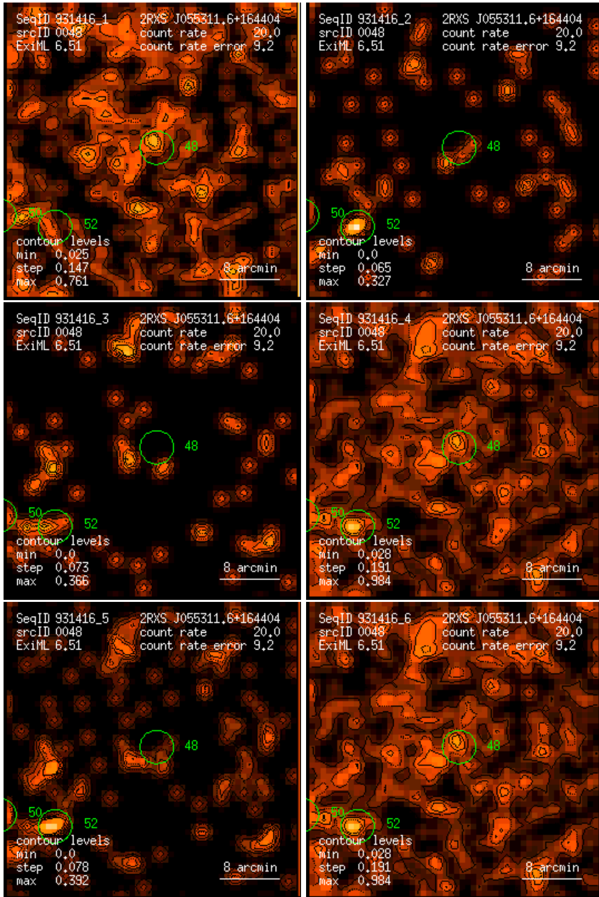
Figure 48: RASS 931416: detection 0048: band rate images, Gaussian filter: (1) PSPC channels 11 – 41, (2) 52 – 90, (3) 91 – 201, (4) 11 – 235, (5) 52 – 201, (6) 11 – 201. Broad band rates in counts/ks. Band rate contour levels in counts/ks/arcmin 2 .
