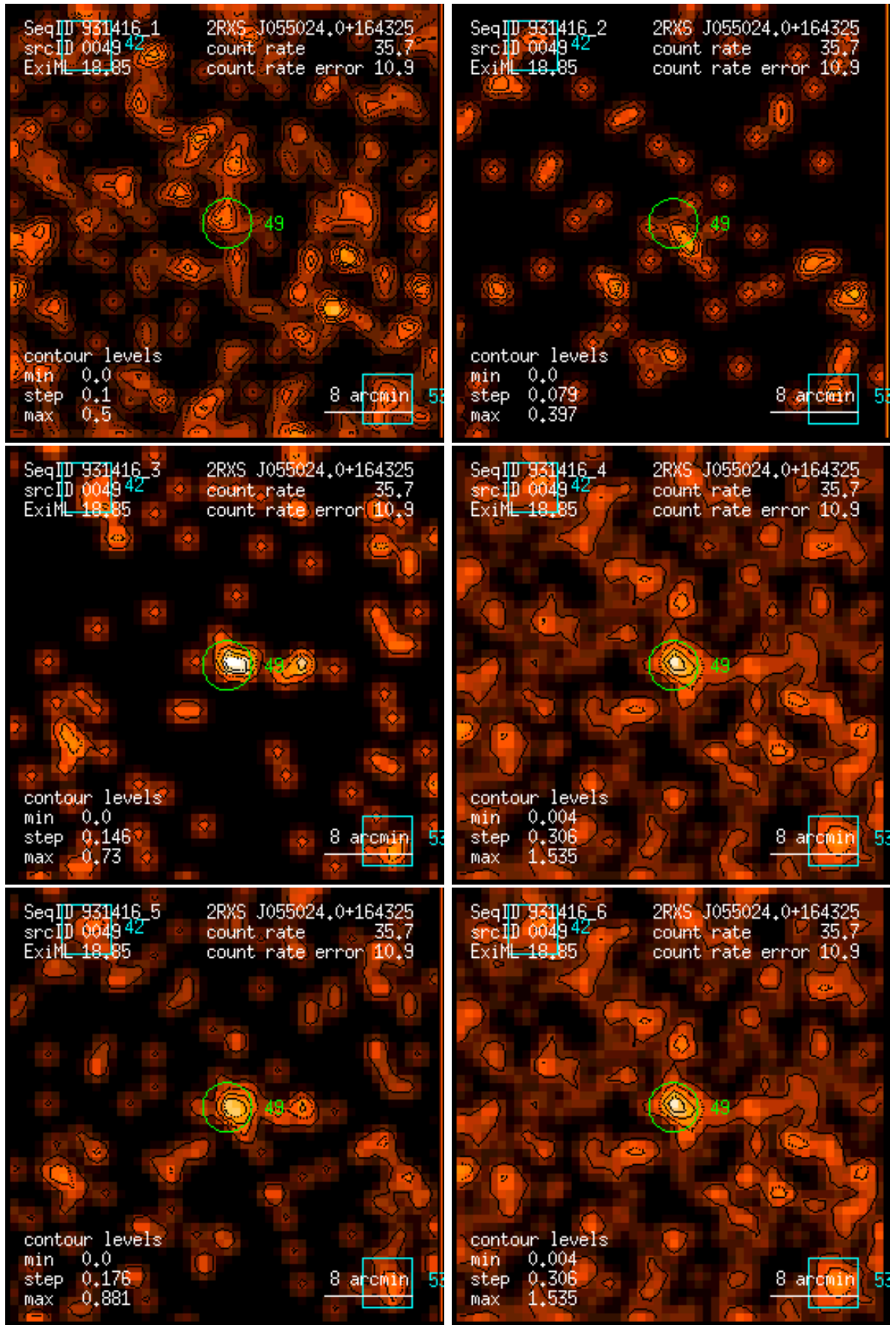
Figure 49: RASS 931416: detection 0049: band rate images, Gaussian filter: (1) PSPC channels 11 – 41, (2) 52 – 90, (3) 91 – 201, (4) 11 – 235, (5) 52 – 201, (6) 11 – 201. Broad band rates in counts/ks. Band rate contour levels in counts/ks/arcmin 2 .
