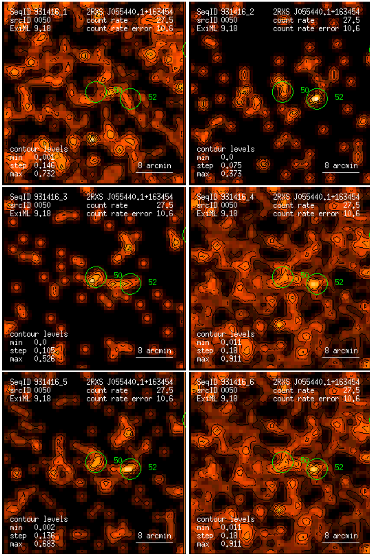
Figure 50: RASS 931416: detection 0050: band rate images, Gaussian filter: (1) PSPC channels 11 – 41, (2) 52 – 90, (3) 91 – 201, (4) 11 – 235, (5) 52 – 201, (6) 11 – 201. Broad band rates in counts/ks. Band rate contour levels in counts/ks/arcmin 2 .
