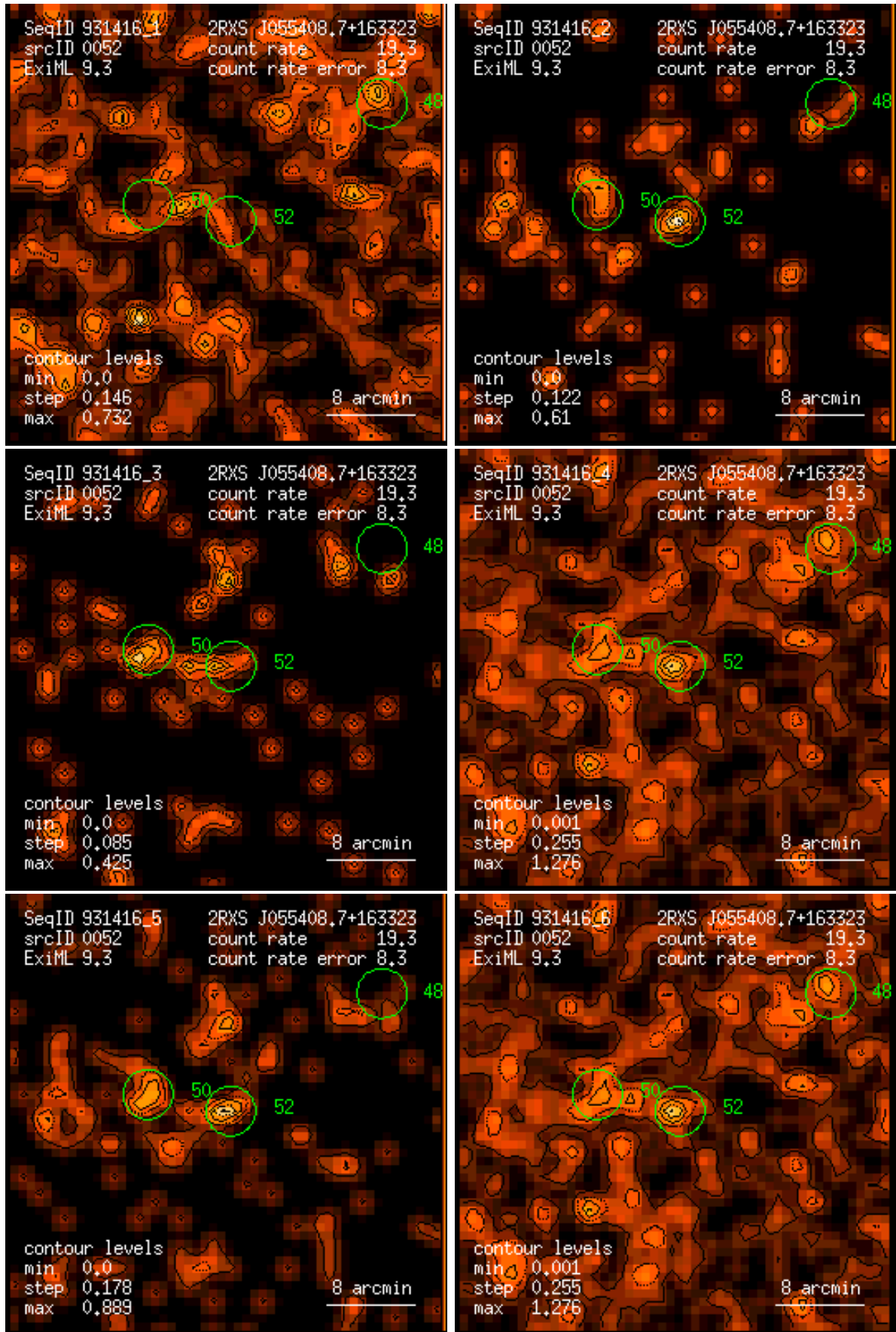
Figure 52: RASS 931416: detection 0052: band rate images, Gaussian filter: (1) PSPC channels 11 – 41, (2) 52 – 90, (3) 91 – 201, (4) 11 – 235, (5) 52 – 201, (6) 11 – 201. Broad band rates in counts/ks. Band rate contour levels in counts/ks/arcmin 2 .
