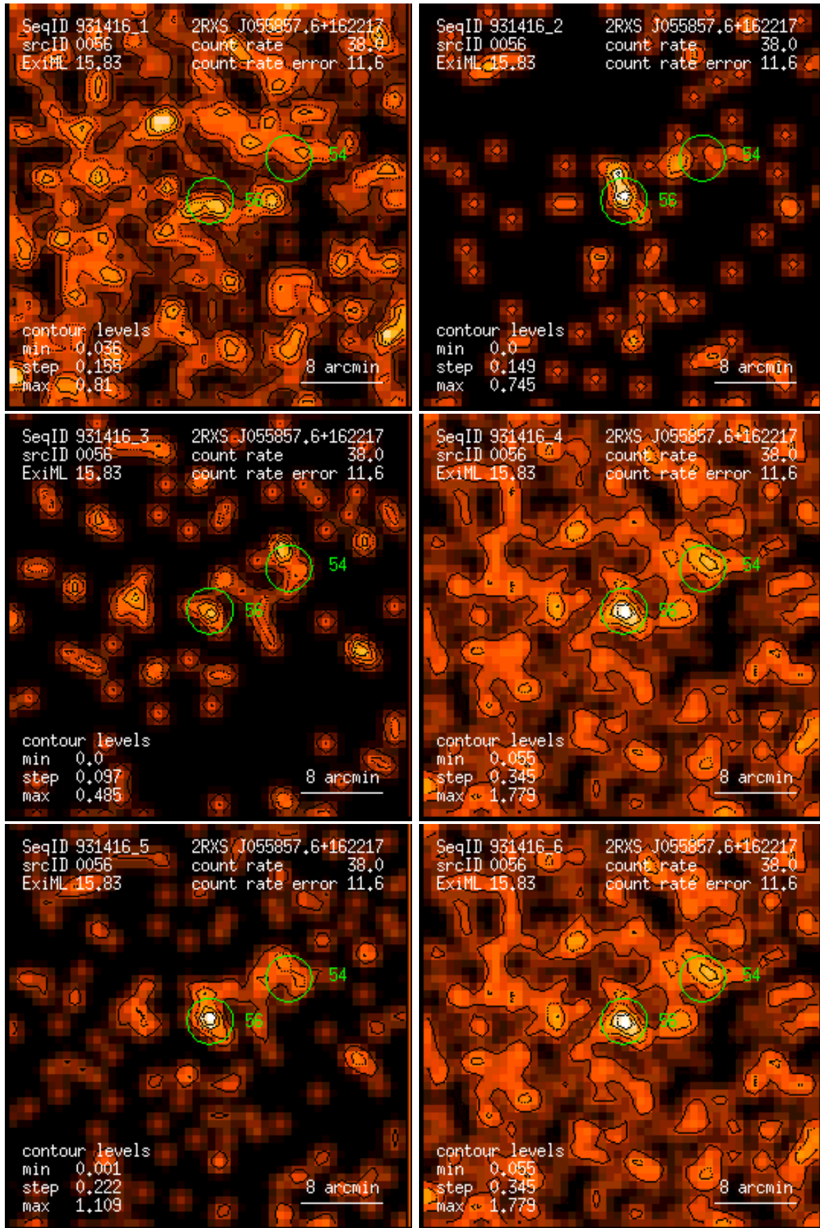
Figure 56: RASS 931416: detection 0056: band rate images, Gaussian filter: (1) PSPC channels 11 – 41, (2) 52 – 90, (3) 91 – 201, (4) 11 – 235, (5) 52 – 201, (6) 11 – 201. Broad band rates in counts/ks. Band rate contour levels in counts/ks/arcmin 2 .
