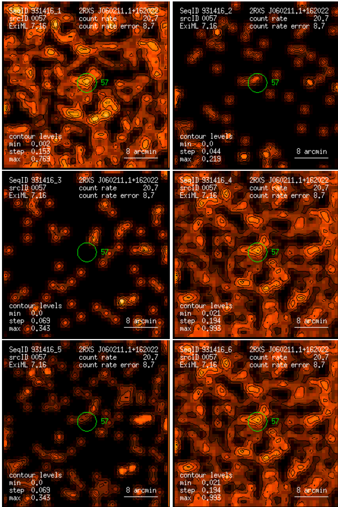
Figure 57: RASS 931416: detection 0057: band rate images, Gaussian filter: (1) PSPC channels 11 – 41, (2) 52 – 90, (3) 91 – 201, (4) 11 – 235, (5) 52 – 201, (6) 11 – 201. Broad band rates in counts/ks. Band rate contour levels in counts/ks/arcmin 2 .
