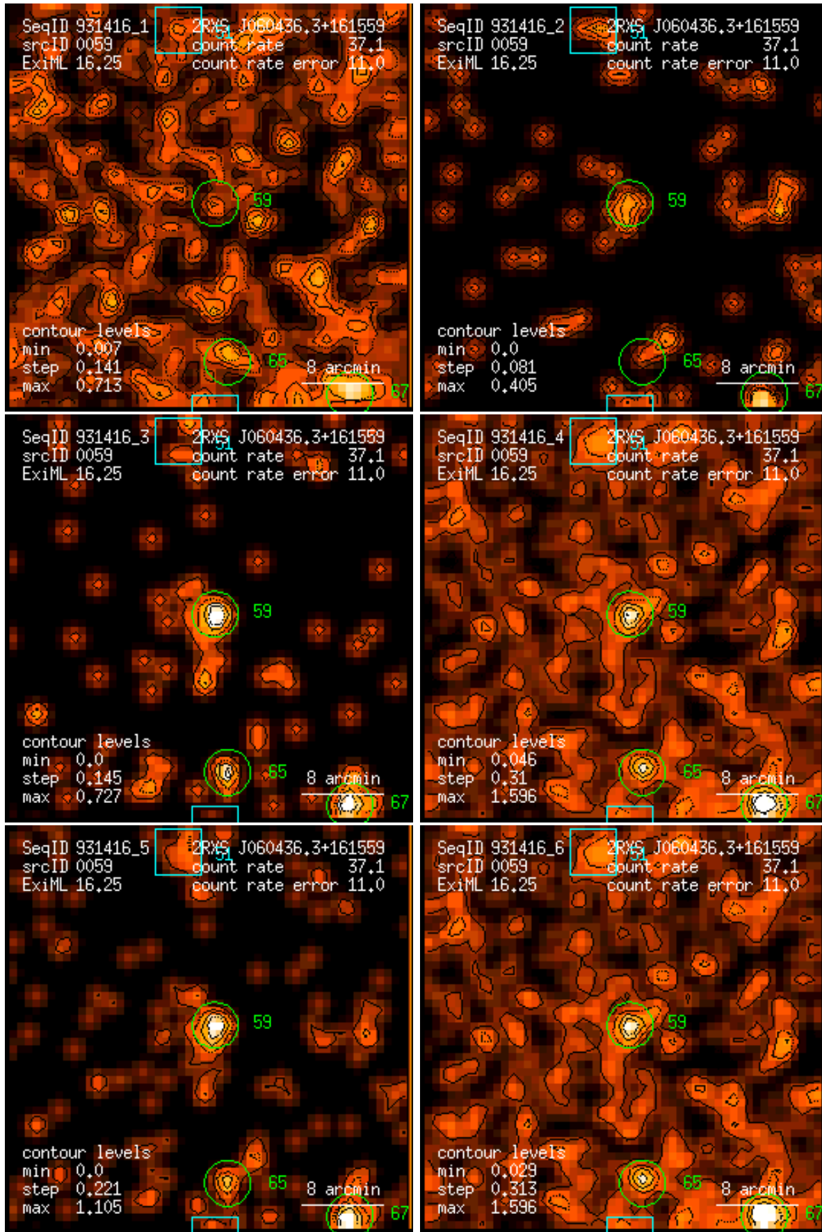
Figure 59: RASS 931416: detection 0059: band rate images, Gaussian filter: (1) PSPC channels 11 – 41, (2) 52 – 90, (3) 91 – 201, (4) 11 – 235, (5) 52 – 201, (6) 11 – 201. Broad band rates in counts/ks. Band rate contour levels in counts/ks/arcmin 2 .
