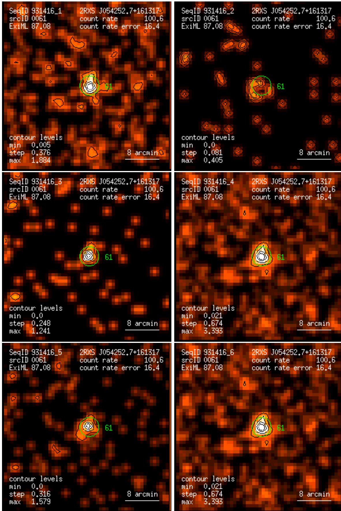
Figure 61: RASS 931416: detection 0061: band rate images, Gaussian filter: (1) PSPC channels 11 – 41, (2) 52 – 90, (3) 91 – 201, (4) 11 – 235, (5) 52 – 201, (6) 11 – 201. Broad band rates in counts/ks. Band rate contour levels in counts/ks/arcmin 2 .
