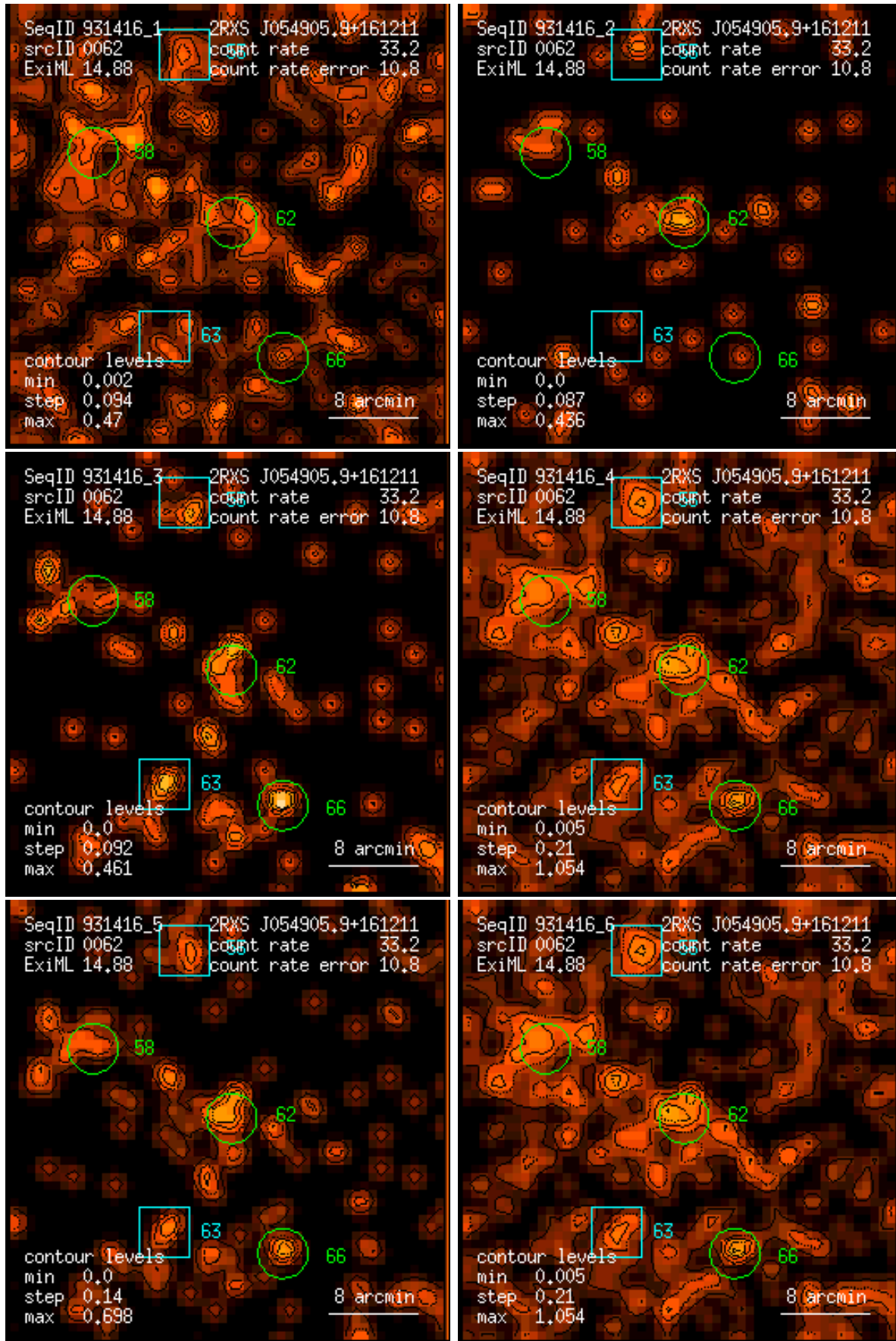
Figure 62: RASS 931416: detection 0062: band rate images, Gaussian filter: (1) PSPC channels 11 – 41, (2) 52 – 90, (3) 91 – 201, (4) 11 – 235, (5) 52 – 201, (6) 11 – 201. Broad band rates in counts/ks. Band rate contour levels in counts/ks/arcmin 2 .
