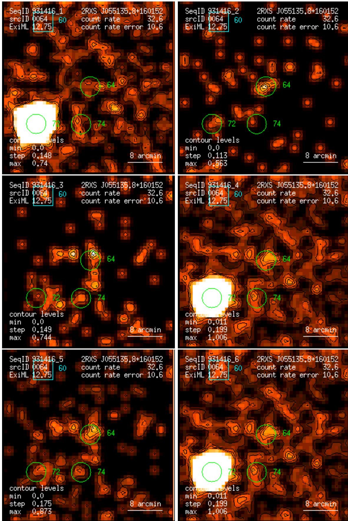
Figure 64: RASS 931416: detection 0064: band rate images, Gaussian filter: (1) PSPC channels 11 – 41, (2) 52 – 90, (3) 91 – 201, (4) 11 – 235, (5) 52 – 201, (6) 11 – 201. Broad band rates in counts/ks. Band rate contour levels in counts/ks/arcmin 2 .
